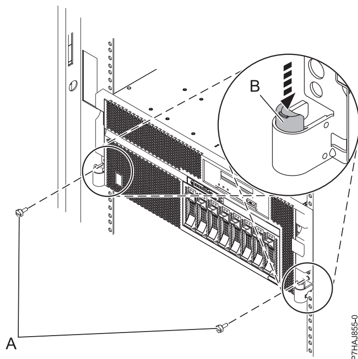
Figura 24. Liberando as Travas do Rack
