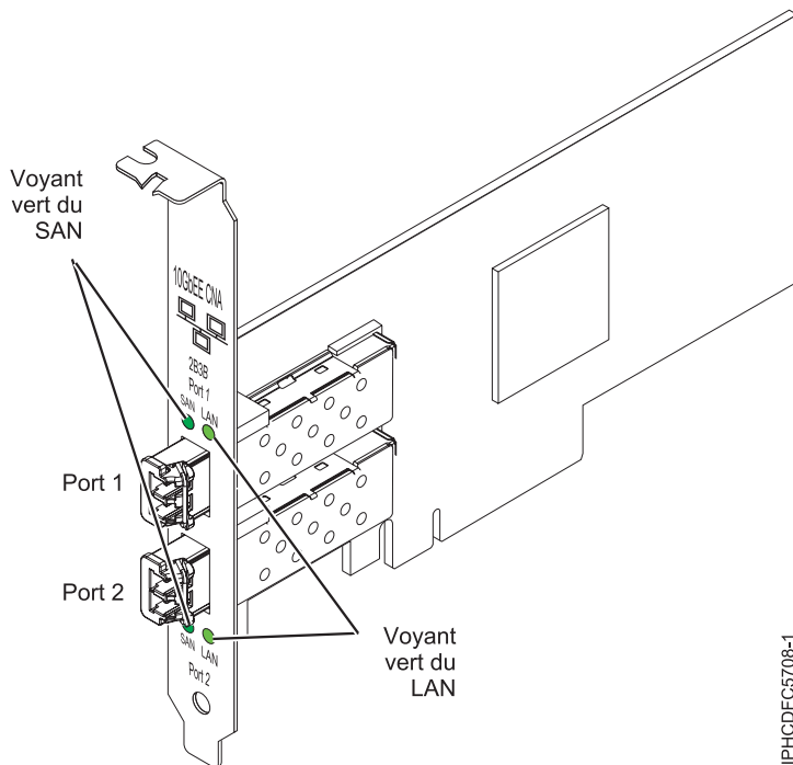
Figure 22. carte double port PCIe FCoE 10 Gb
