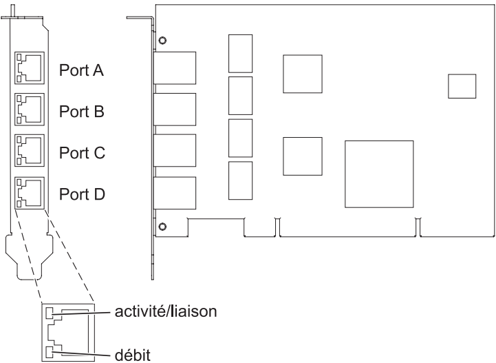
Figure 30. Carte PCI-X 4 ports 10/100/1000 Base-TX
