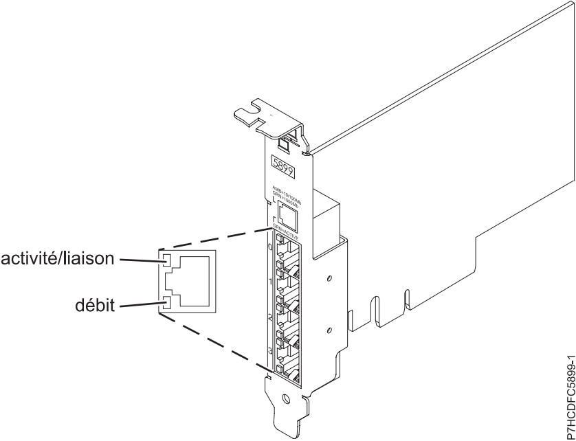
Figure 35. Carte
