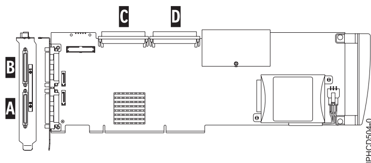
Figure 53. Carte RAID SCSI PCI-X DDR double canal Ultra320
