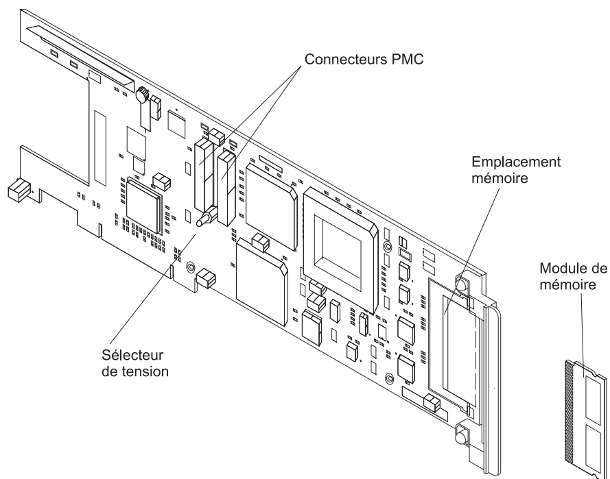
Figure 60. Carte PCI de base IBM ARTIC960Hx
