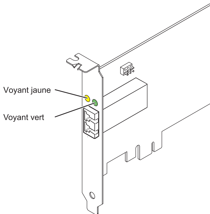
Figure 9. Adaptateur 5773
