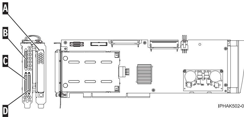
Figure 58. Adaptateur 5782
