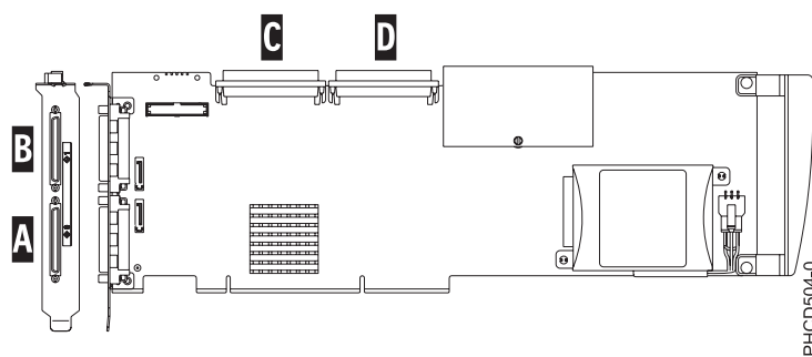
Figure 71. Carte RAID SCSI PCI-X DDR double canal Ultra320
