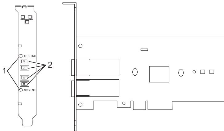
Figure 40. PCI Express Gigabit Ethernet SX 2 ports
