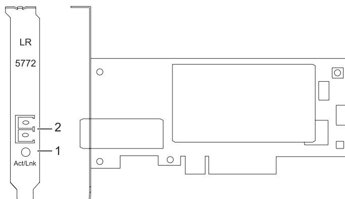
Figure 42. Carte PCI Express Ethernet-LR 10 gigabits
