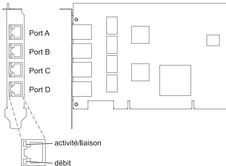
Figure 38. Carte PCI-X 4 ports 10/100/1000 Base-TX
