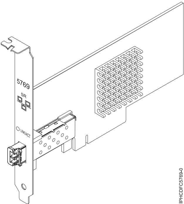
Figure 41. carte PCIe 10 Gigabit Ethernet-SR
