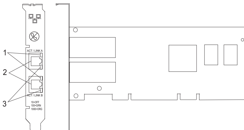
Figure 29. Adaptateur 2 ports 10/100/1000 Base-TX Ethernet PCI-X
