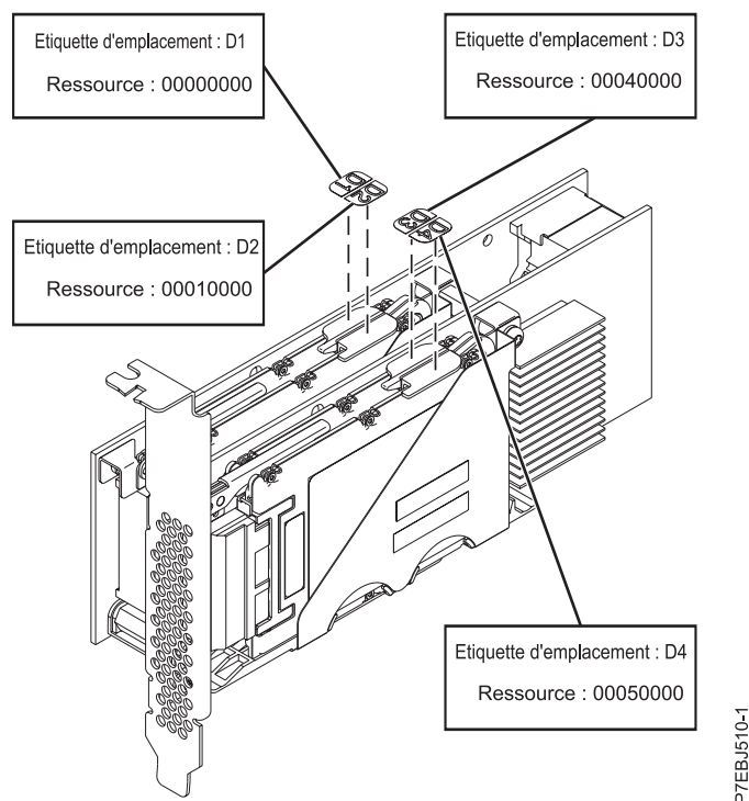
Figure 50. Carte SAS RAID PCIe Dual - x4 3 gigabits
