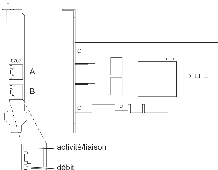
Figure 39. Carte PCI Express Ethernet 10/100/1000 Base-TX 2 ports
