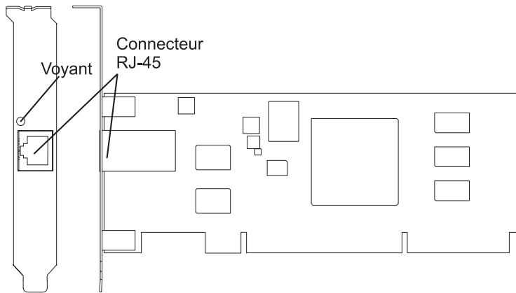
Figure 32. Carte PCI-X TOE iSCSI TX 1 Gbit
