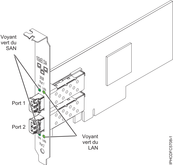
Figure 24. carte PCIe LP 10 gigabits FCoE 2 ports
