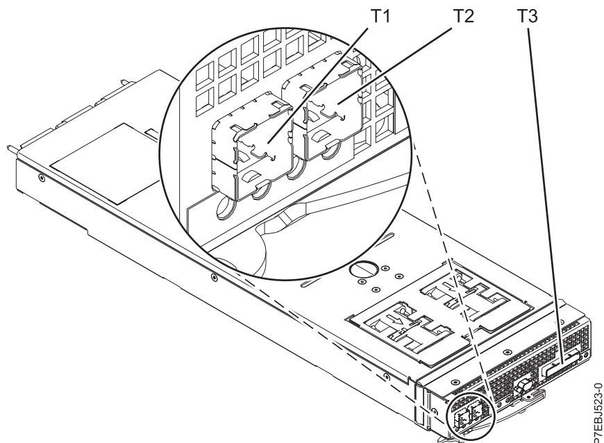
Figure 58. CCIN 57C3 - Boîtier SAS RAID cache PCIe2 3,1 Go 6 gigabits x8.
