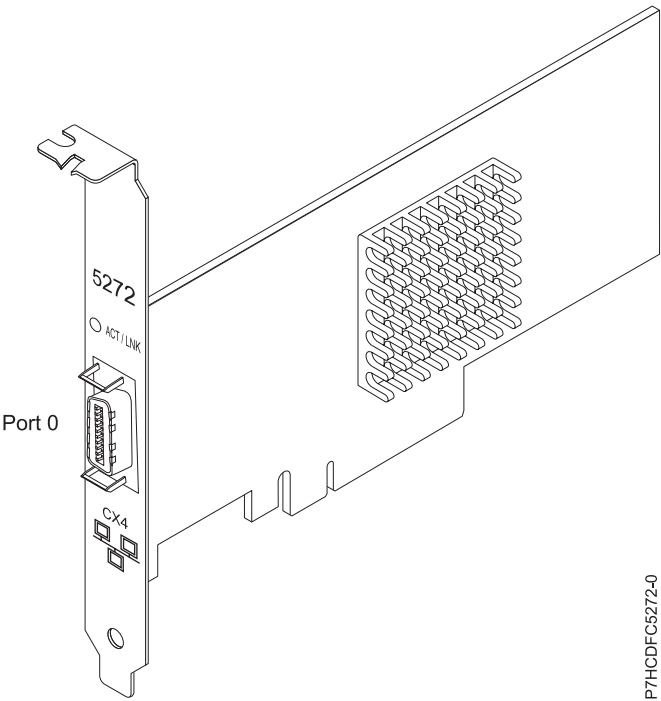
Figure 26. carte PCIe LP 10GbE CX4 1 port
