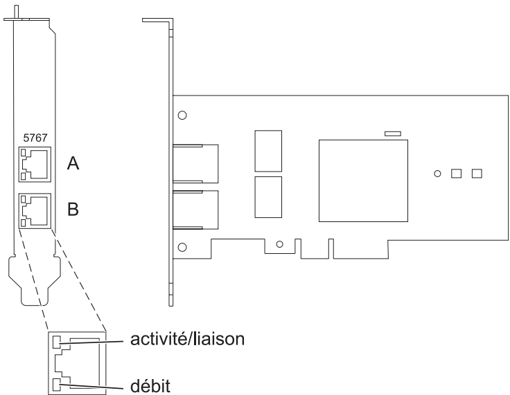
Figure 32. Carte PCI Express Ethernet 10/100/1000 Base-TX 2 ports
