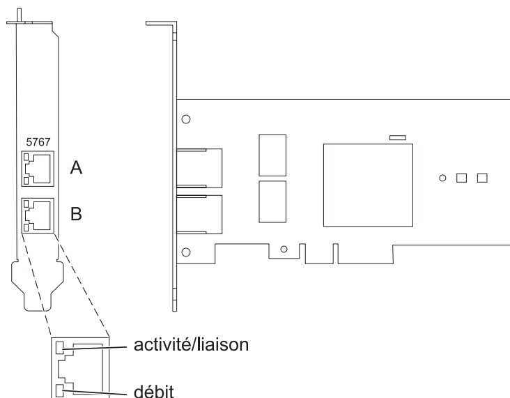
Figure 38. Carte PCI Express Ethernet 10/100/1000 Base-TX 2 ports
