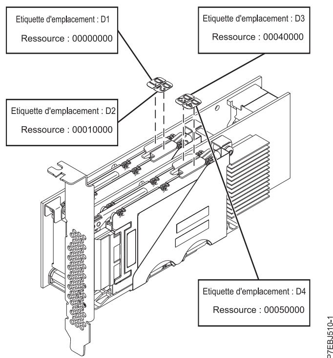
Figure 52. Carte SAS RAID PCIe Dual - x4 3 gigabits
