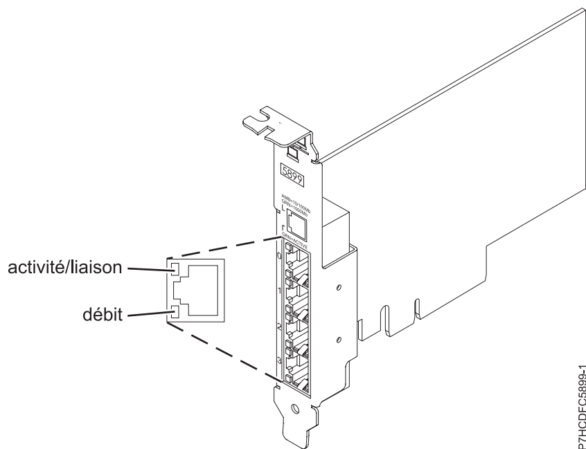
Figure 42. Carte
