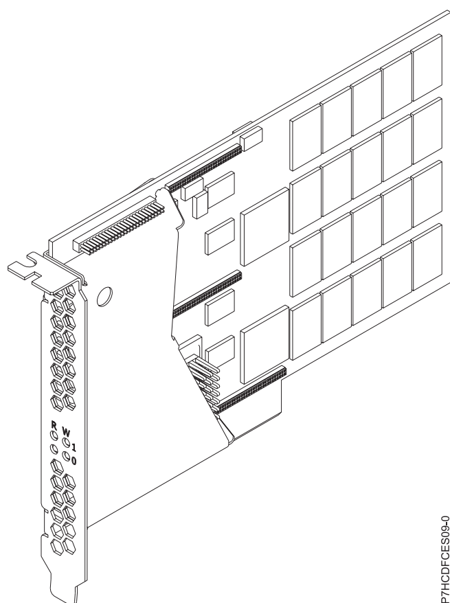
Figure 59. IBM Flash Adapter 90 (PCIe2 0.9TB)
