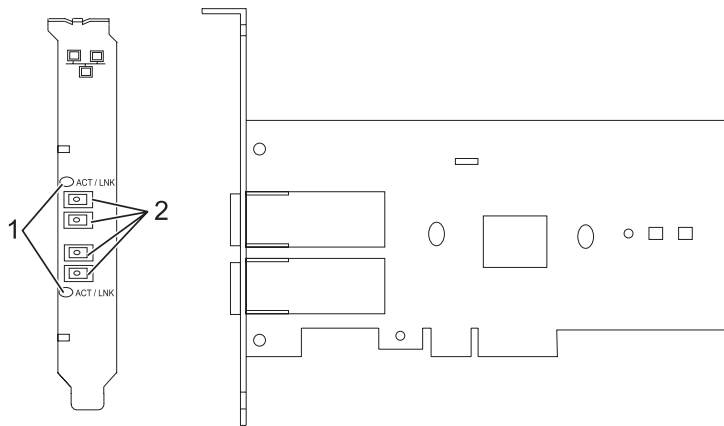
Figure 39. PCI Express Gigabit Ethernet SX 2 ports
