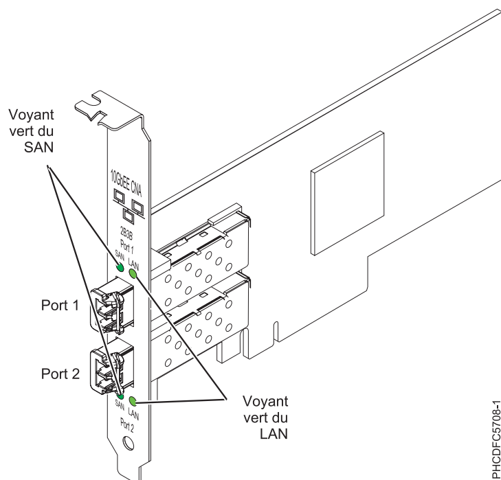
Figure 35. carte double port PCIe FCoE 10 Gb
