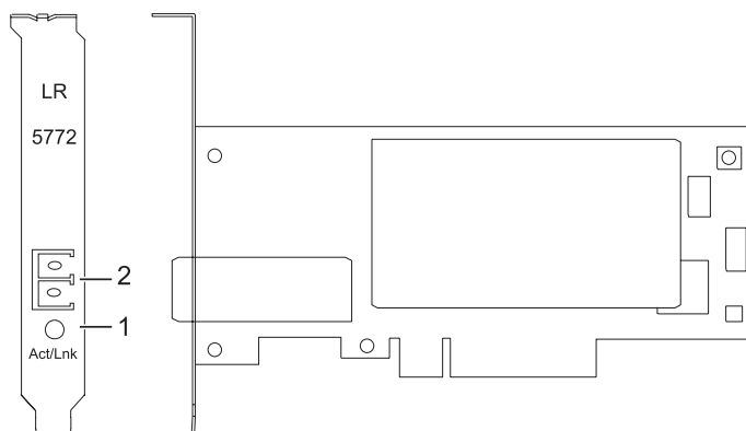
Figure 41. Carte PCI Express Ethernet-LR 10 gigabits
