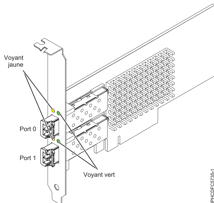
Figure 9. Carte EN0B
