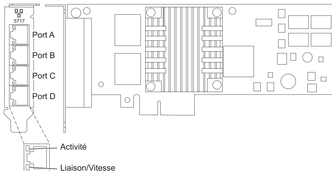
Figure 36. Carte PCIe 10/100/1000 Base-TX 4 ports
