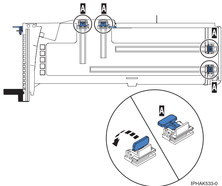
Figure 76. Crochets de retenue
