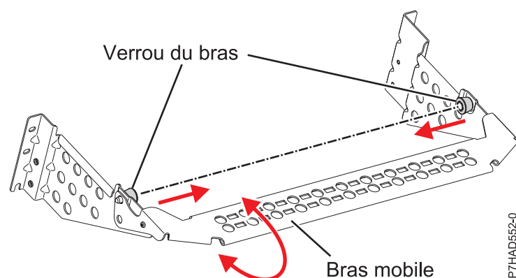
Figure 136. Passe-câbles
