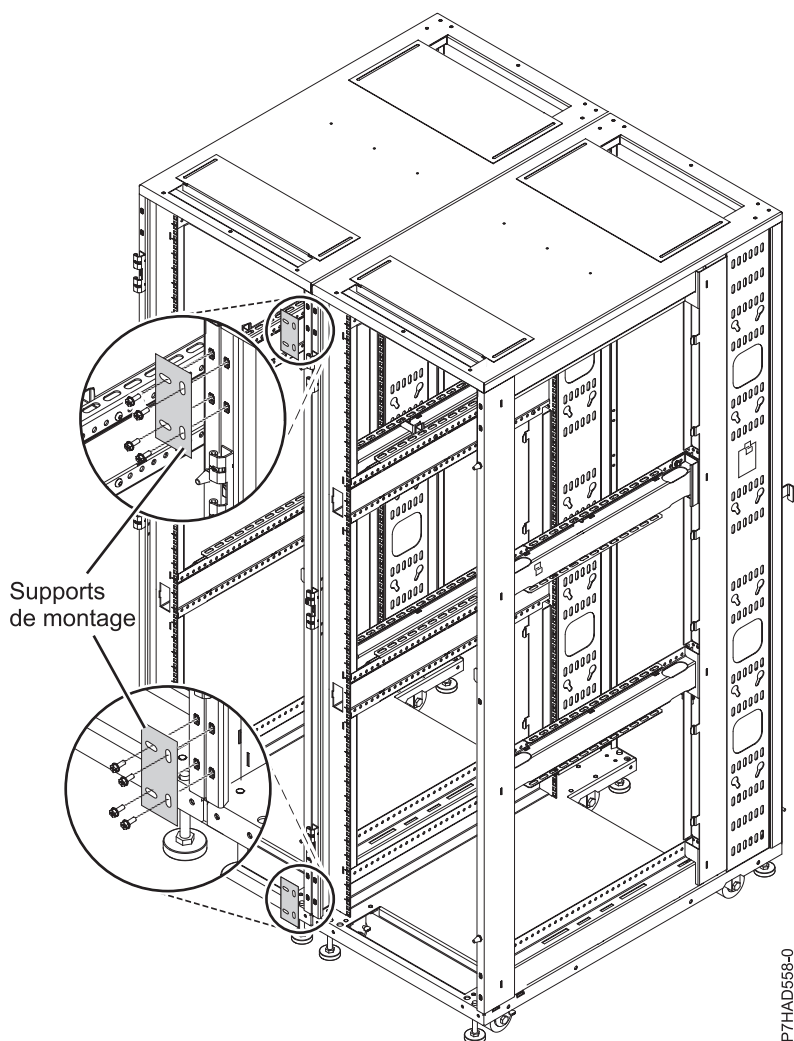
Figure 28. Supports de montage
