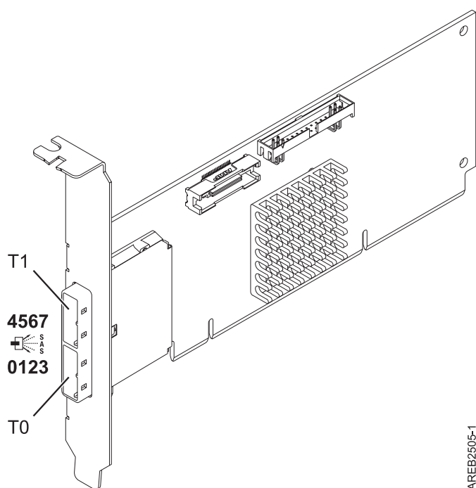
Figure 1. CCIN 572A : carte SAS PCI-X 266 External Dual-x4 3 Go
