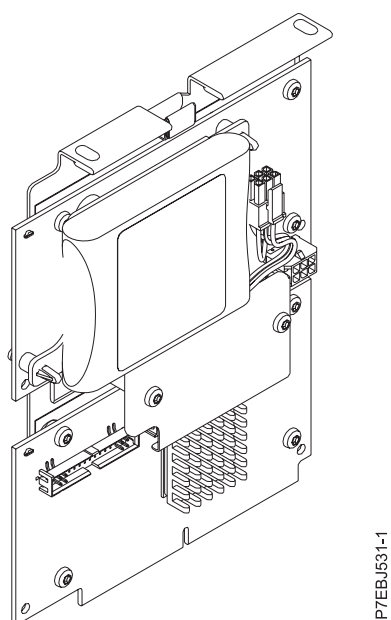
Figure 14. CCIN 2BD9 - Carte SAS RAID PCI-X266 Planar 3 Go
