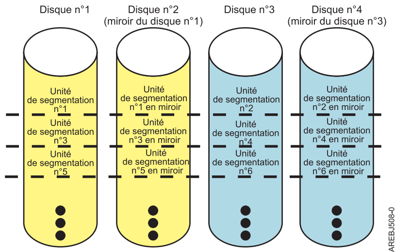
Figure 21. RAID 10
