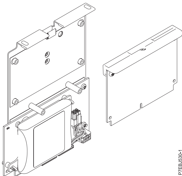
Figure 13. CCIN 2BE0 - Carte SAS PCI-X266 Planar 3 Go
