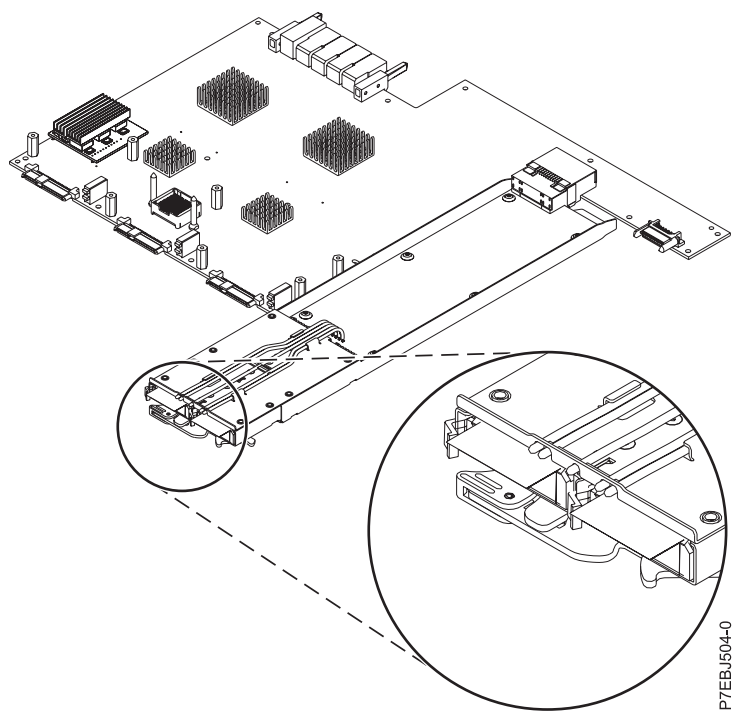
Figure 12. CCIN 57CF - Carte SAS RAID PCI Express x8 Planar 3 Go
