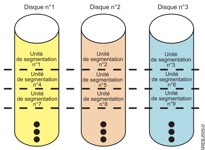
Figure 18. RAID 0
