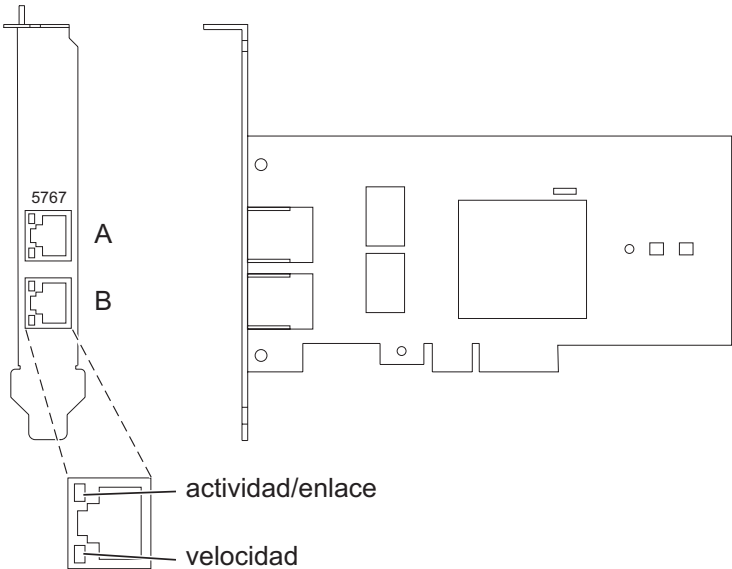
Figura 58. Adaptador PCI Express Ethernet Base-TX 10/100/1000 de 2 puertos
