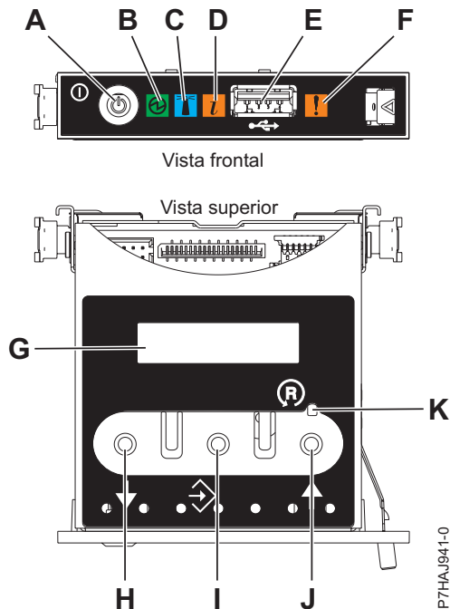
Figura 2. Panel de control
