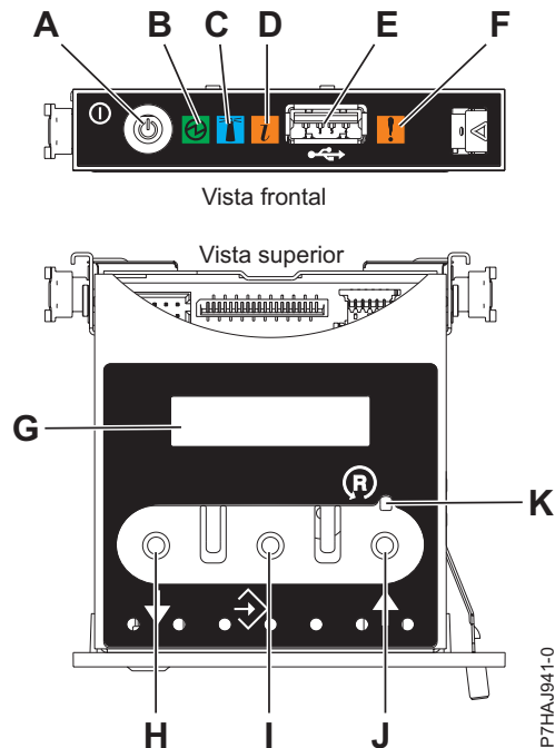
Figura 2. Panel de control
