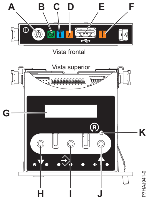
Figura 19. Panel de control
