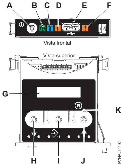
Figura 18. Panel de control
