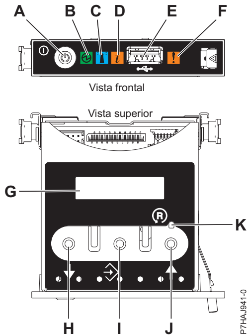
Figura 14. Panel de control
