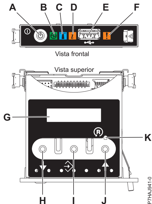
Figura 13. Panel de control
