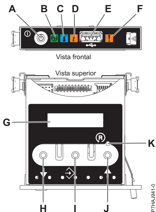
Figura 94. Panel de control
