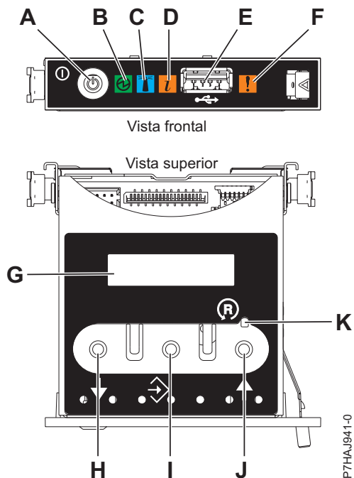
Figura 107. Panel de control
