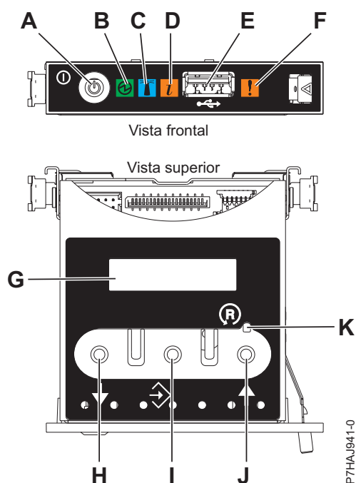
Figura 106. Panel de control
