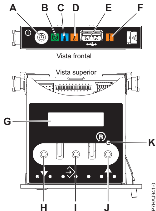
Figura 59. Panel de control
