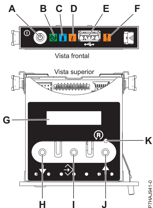
Figura 1. Panel de control
