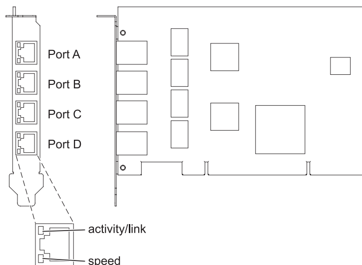
Figura 30. Adaptador PCI-X 4 Ports 10/100/1000 Base-TX
