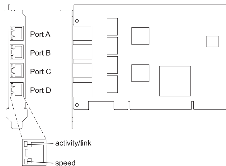
Figura 29. Adaptador PCI-X 4 Ports 10/100/1000 Base-TX
