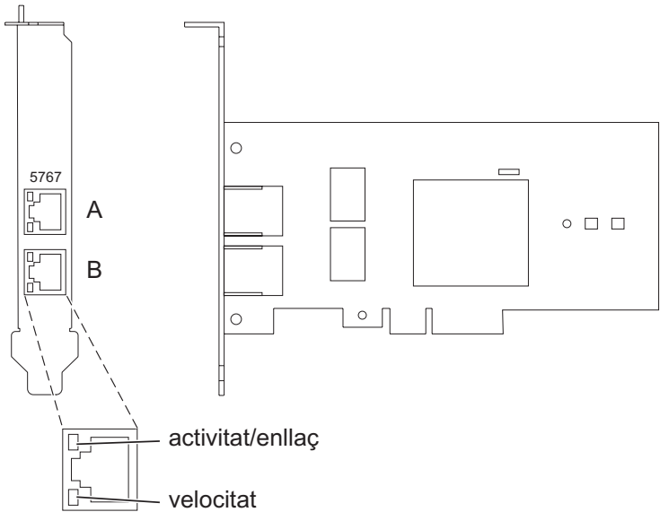
Figura 31. Adaptador 10/100/1000 Base-TX Ethernet PCI Express de 2 ports
