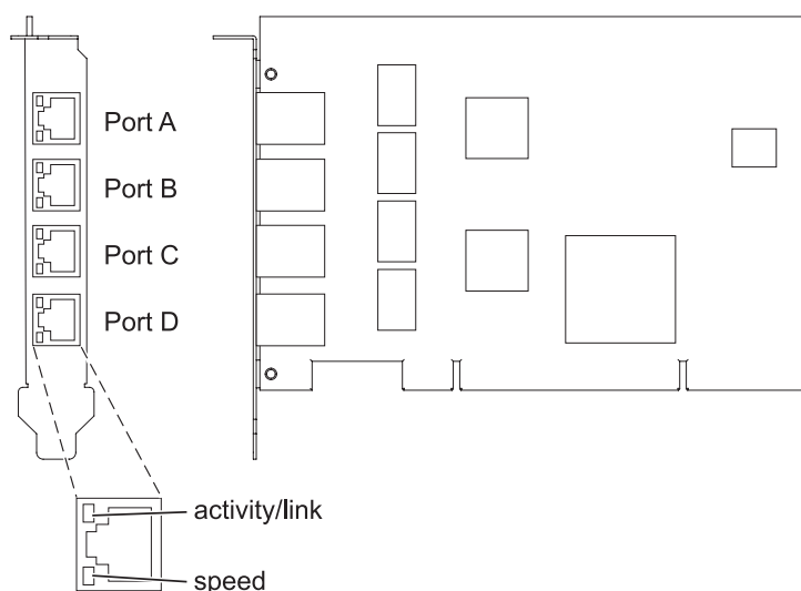
Figura 54. Adaptador PCI-X 4 Ports 10/100/1000 Base-TX
