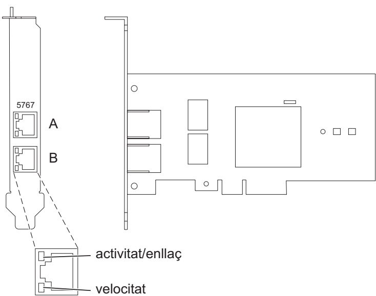
Figura 58. Adaptador 10/100/1000 Base-TX Ethernet PCI Express de 2 ports
