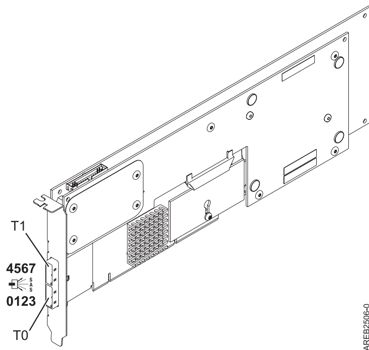
Figura 86. adaptador PCI-X DDR port x4 dual SAS RAID
