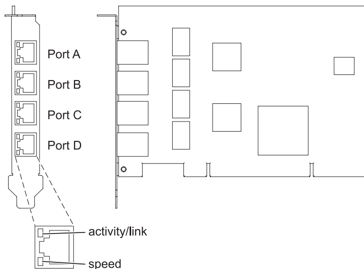
Figura 53. Adaptador PCI-X 4 Ports 10/100/1000 Base-TX
