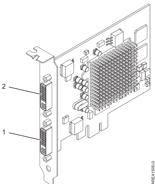
Figura 18. POWER GXT145 PCI Express
