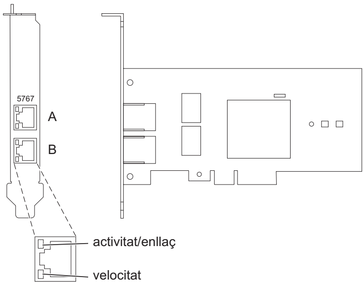
Figura 31. Adaptador 10/100/1000 Base-TX Ethernet PCI Express de 2 ports
