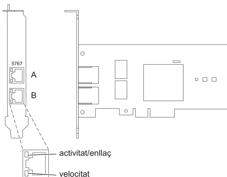
Figura 37. Adaptador 10/100/1000 Base-TX Ethernet PCI Express de 2 ports
