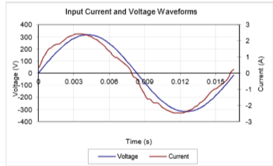
Input AC Current Waveform (ITHD = 8.88%, 50% Load)
