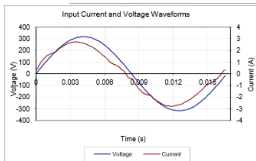
Input AC Current Waveform (ITHD = 5.38%, 50% Load)
