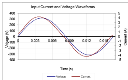
Input AC Current Waveform (THD = 3.91%, 50% Load)
