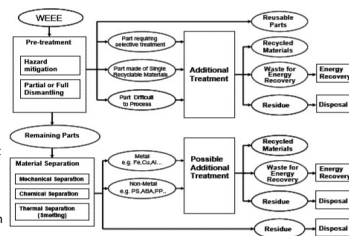
End-of-life treatment processes from IEC/TR 62635
