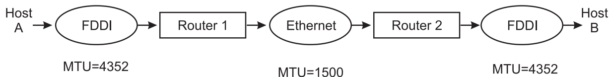
Figure 21. Inter-Subnet Fragmentation. This illustration show a data path from Host A, through an FDDI with an MTU=4352, through Router 1, to the Ethernet with an MTU=1500. From there it goes to Router 2 and another FDDI with an MTU=4352 and out to Host B. An explanation of how fragmentation occurs in this example is described in the text immediately following the illustration.
