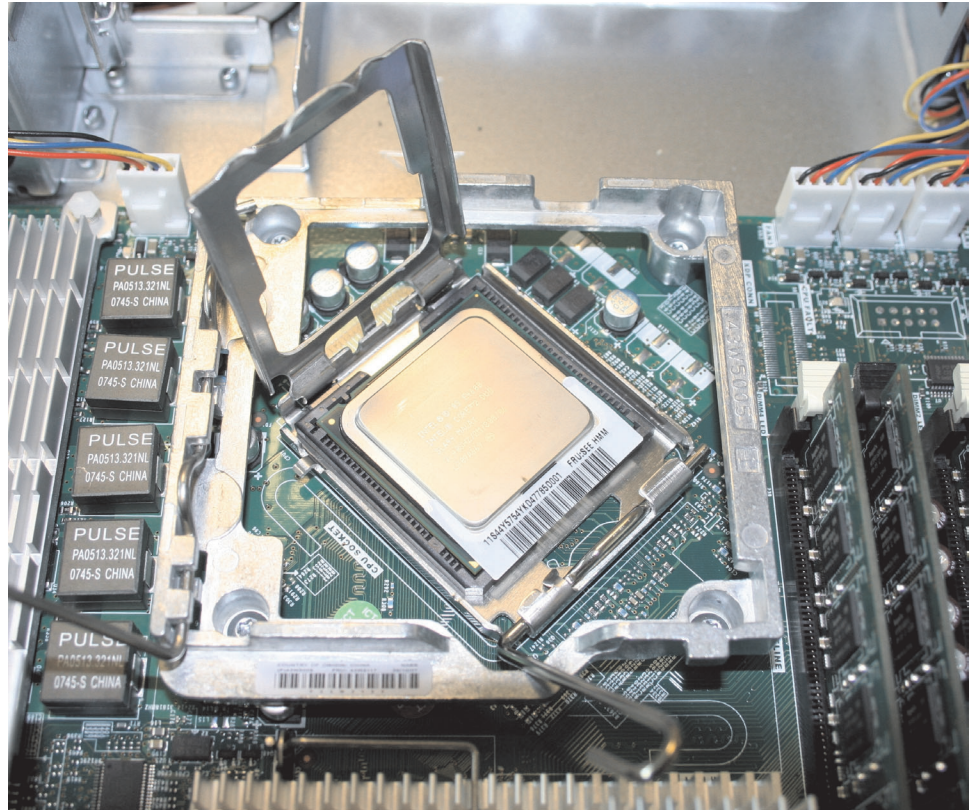
Figure 247. The SAN Volume Controller 2145-8A4 microprocessor bracket frame fully opened
