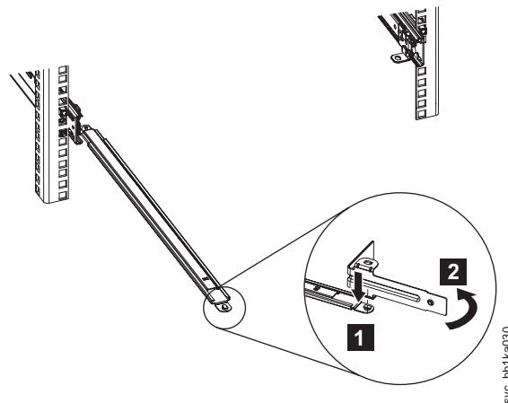
Figure 17. Rack rear: Installing the SAN Volume Controller 2145-CF8 cable-management stop bracket
