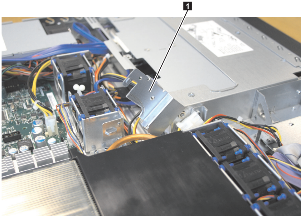
Figure 120. Air deflector for the SAN Volume Controller 2145-8A4 power supply
