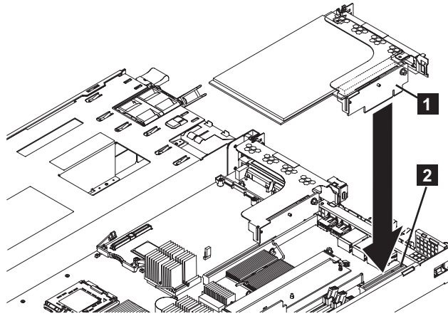
Figure 186. Replacing the riser-card assembly for the SAN Volume Controller 2145-8G4
