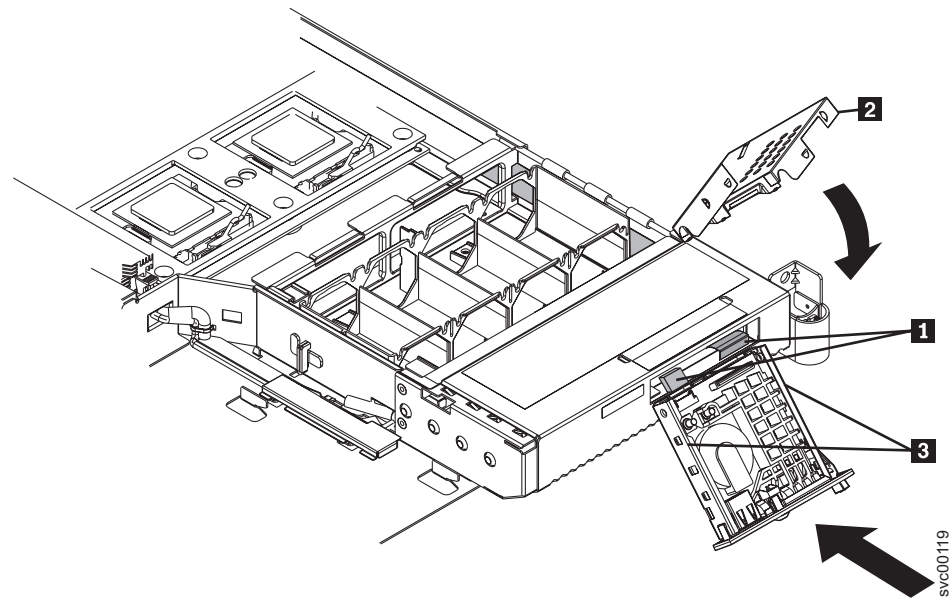
Figure 225. Replacing the operator-information panel
