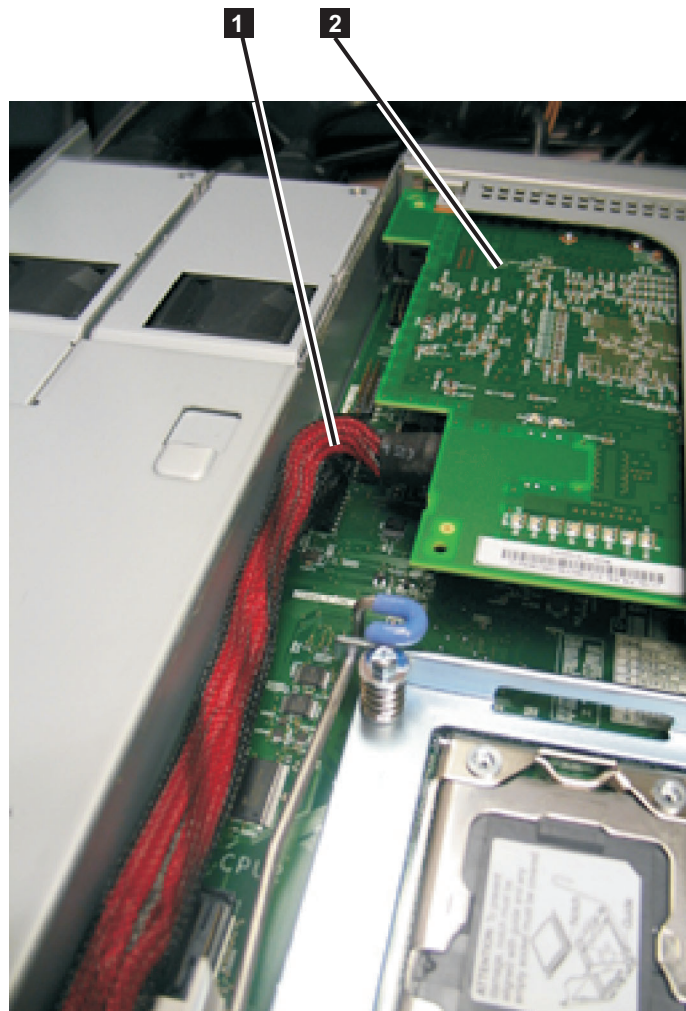
Figure 192. High-speed SAS adapter assembly and high-speed SAS cable in the SAN Volume Controller 2145-CF8
