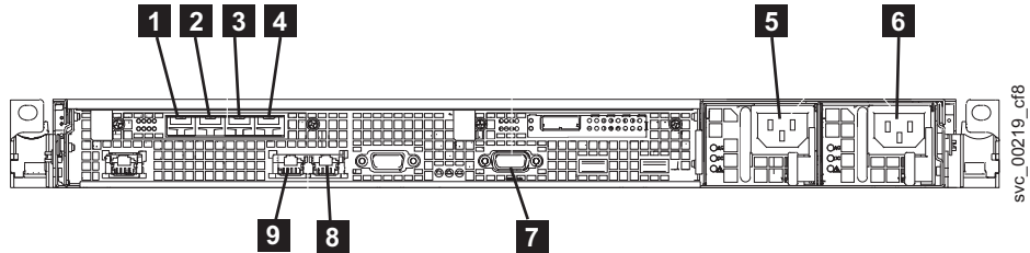
Figure 171. Connectors on the rear of the SAN Volume Controller 2145-CF8
