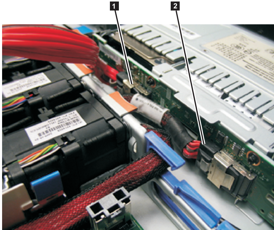
Figure 125. Boot-disk SAS cable and the high-speed SAS cable connected to the disk backplane in the SAN Volume Controller 2145-CF8
