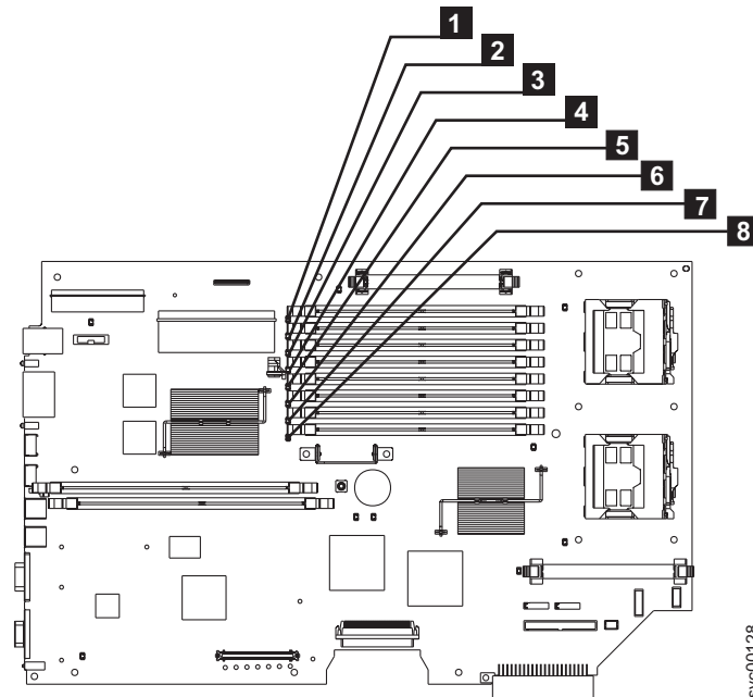
Figure 98. Locating the SAN Volume Controller 2145-8F2 or SAN Volume Controller 2145-8F4 memory modules
