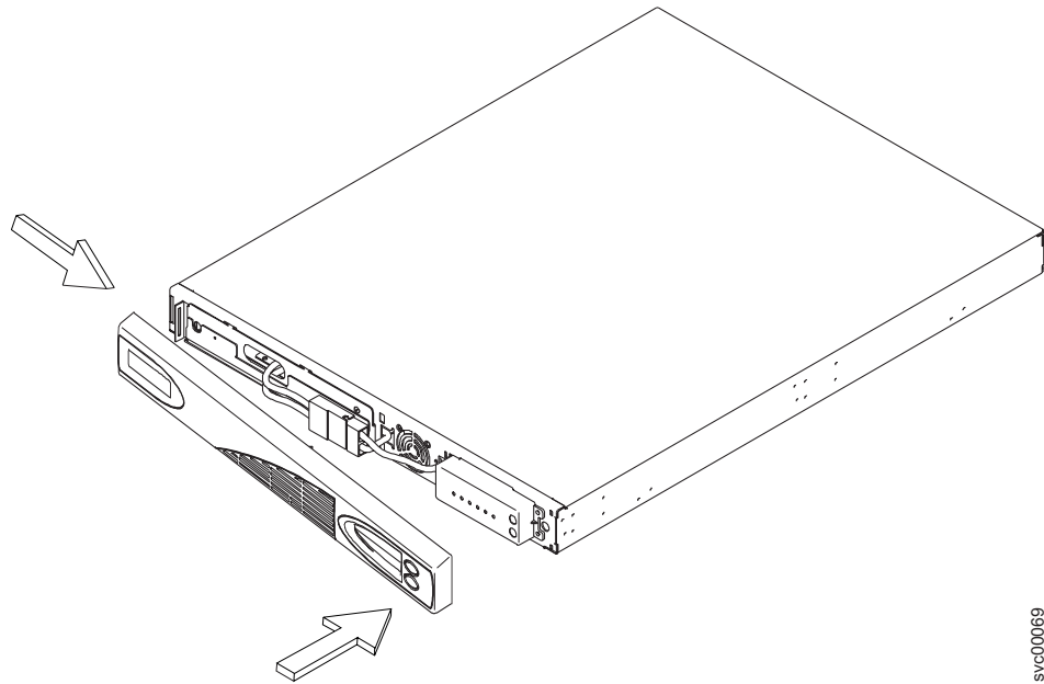
Figure 325. Replacing the 2145 UPS-1U front panel
