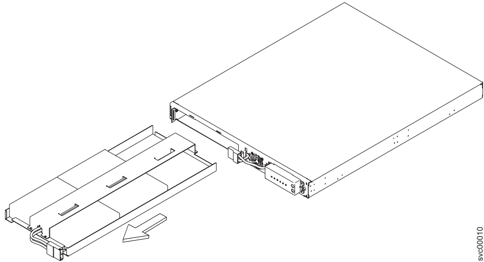
Figure 322. Removing the 2145 UPS-1U battery
