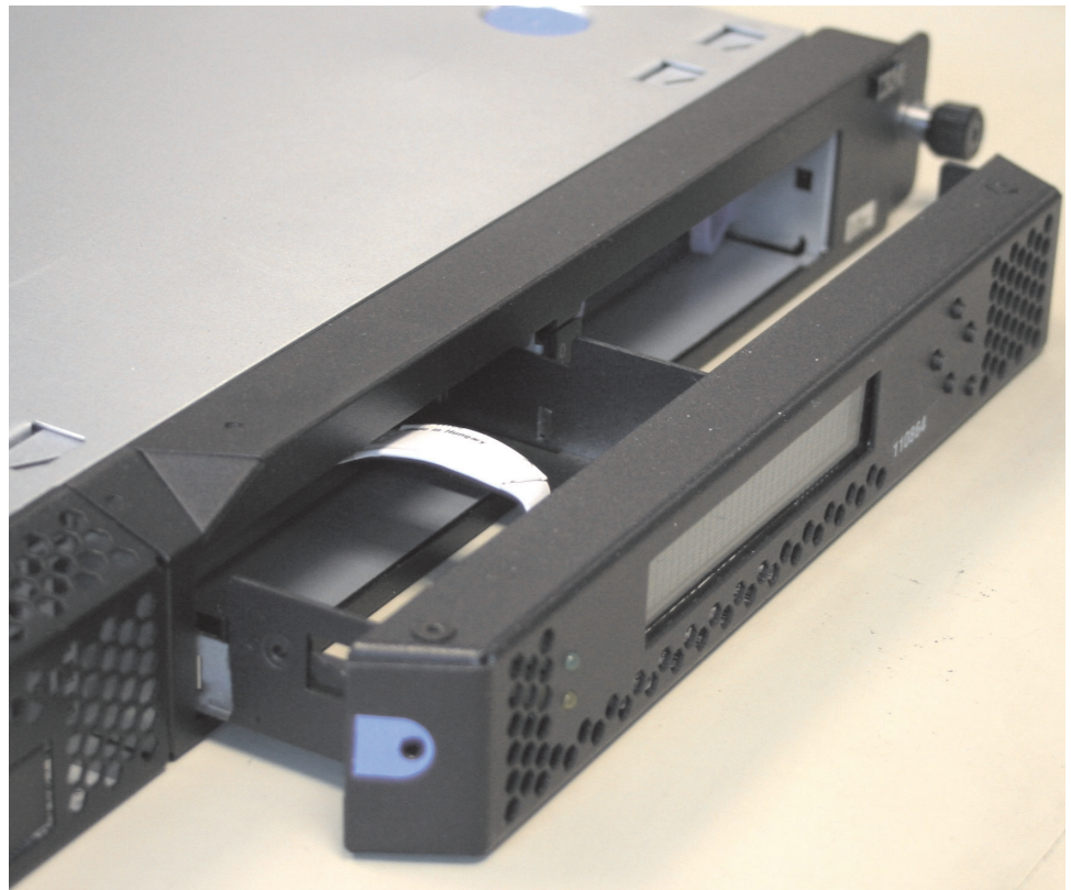
Figure 89. SAN Volume Controller 2145-8A4 service controller
