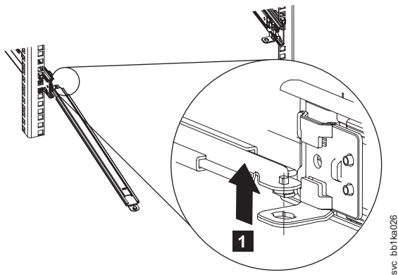
Figure 15. Detaching the SAN Volume Controller 2145-CF8 cable-management support arm
