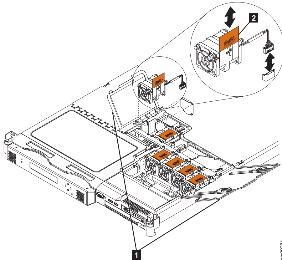
Figure 243. SAN Volume Controller 2145-8G4 fan doors, locations, and connectors
