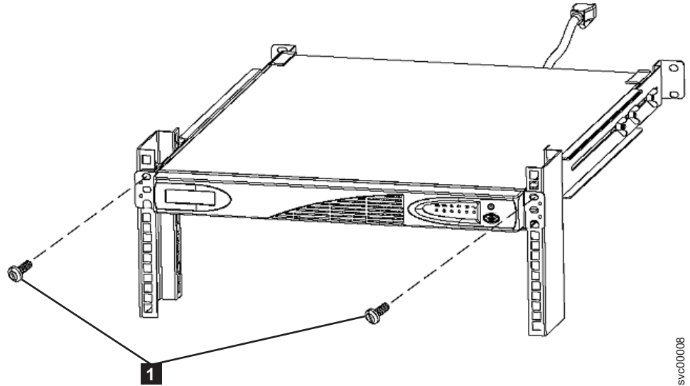
Figure 303. Mounting screws for the 2145 UPS-1U
