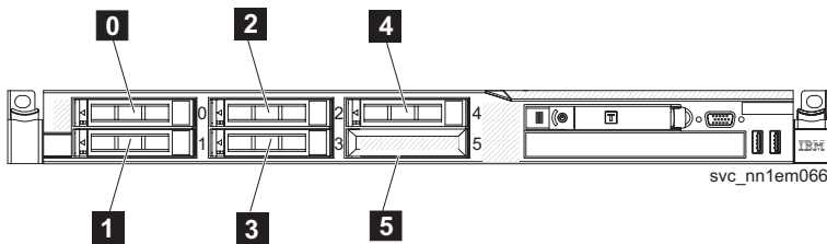
Figure 107. Drive IDs for SAN Volume Controller 2145-CF8
