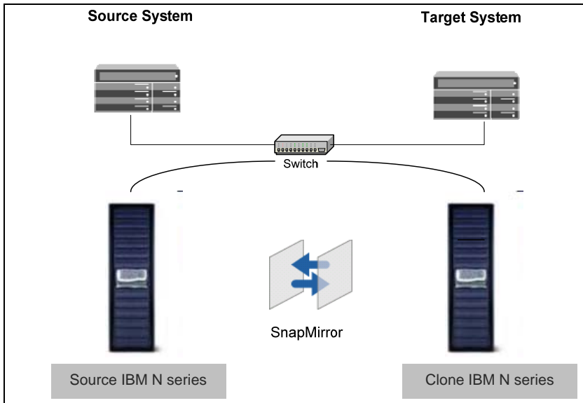
Figure 2) Server and Storage Configuration.
