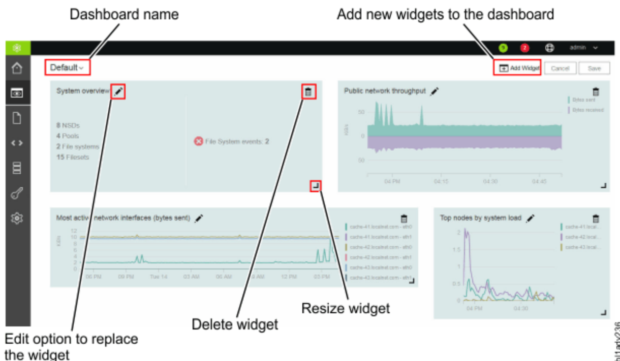
Figure 4. Dashboard page in the edit mode
