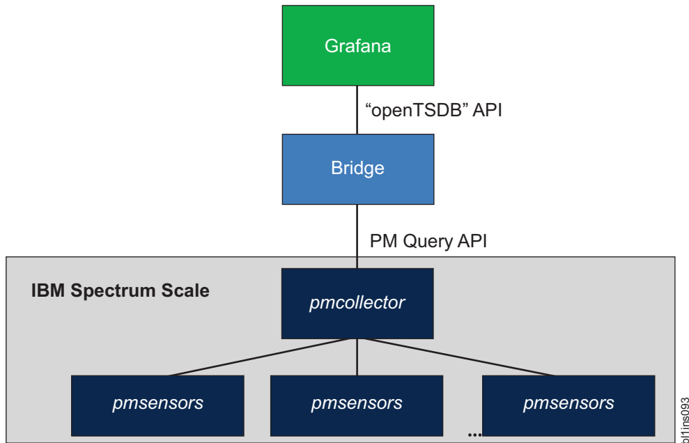
Figure 5. IBM Spectrum Scale integration framework for Grafana
