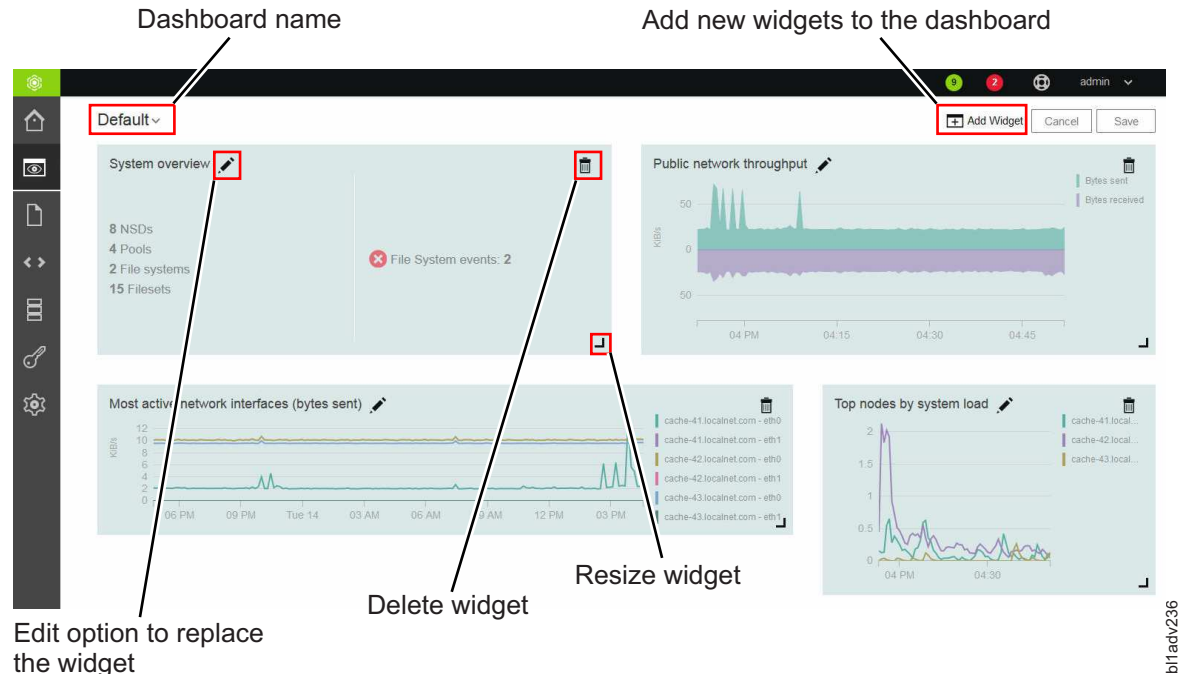
Figure 4. Dashboard page in the edit mode
