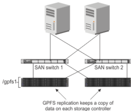
Figure 27. Configuration using GPFS replication for improved availability
