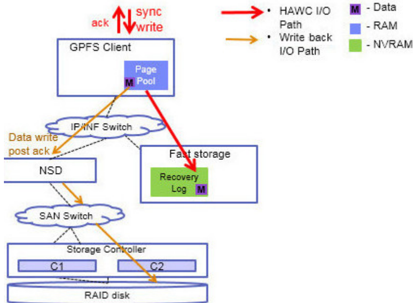
Figure 29. Shared fast storage
