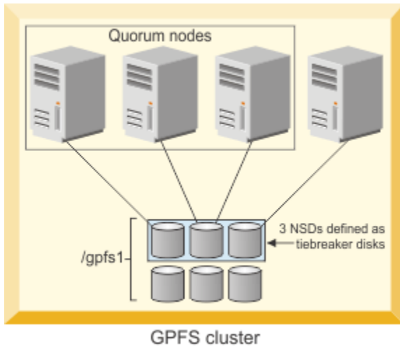
Figure 25. GPFS configuration using node quorum with tiebreaker disks
