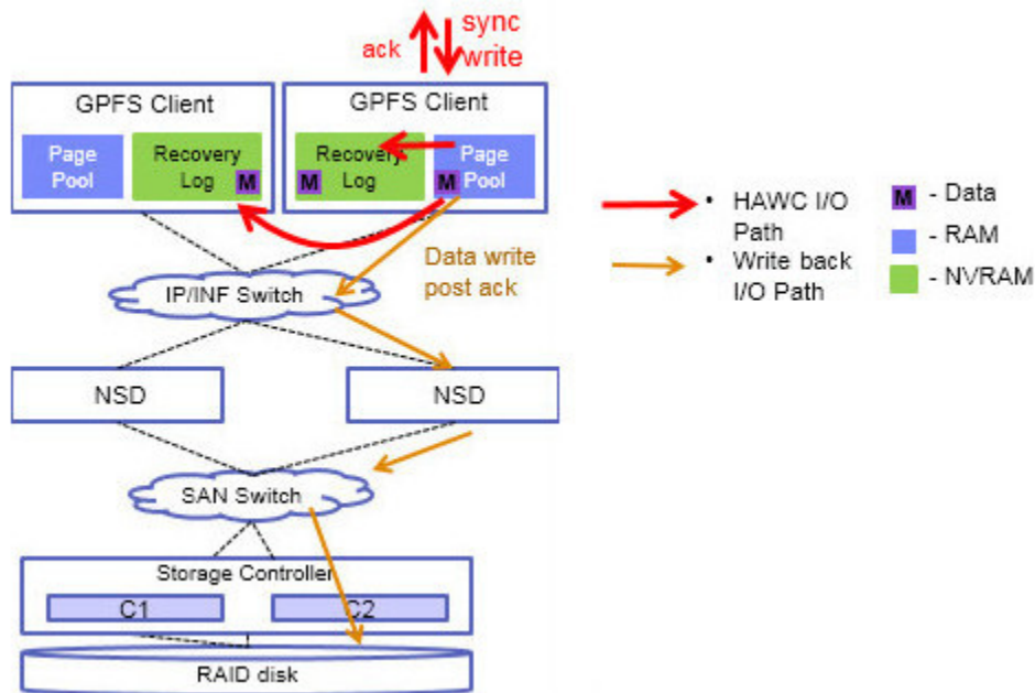
Figure 30. Distributed fast storage
