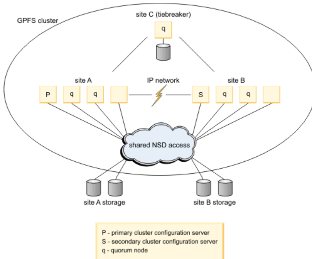
Figure 36. Synchronous mirroring with GPFS replication
