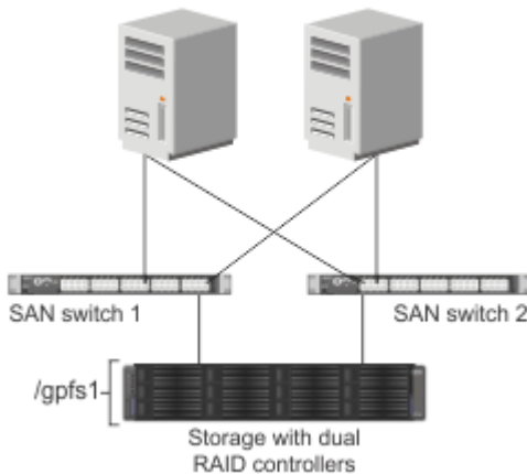
Figure 26. An example of a highly available SAN configuration for a GPFS file system
