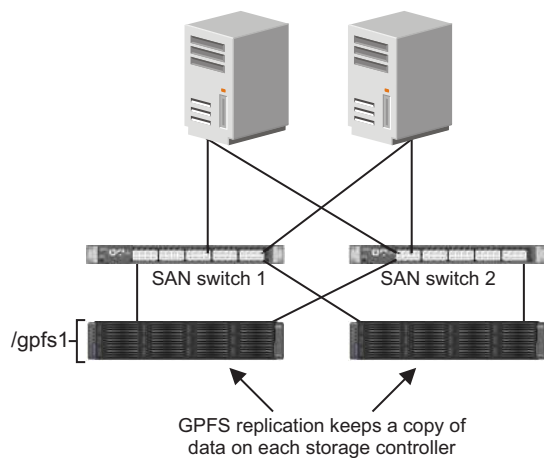
Figure 26. Configuration using GPFS replication for improved availability
