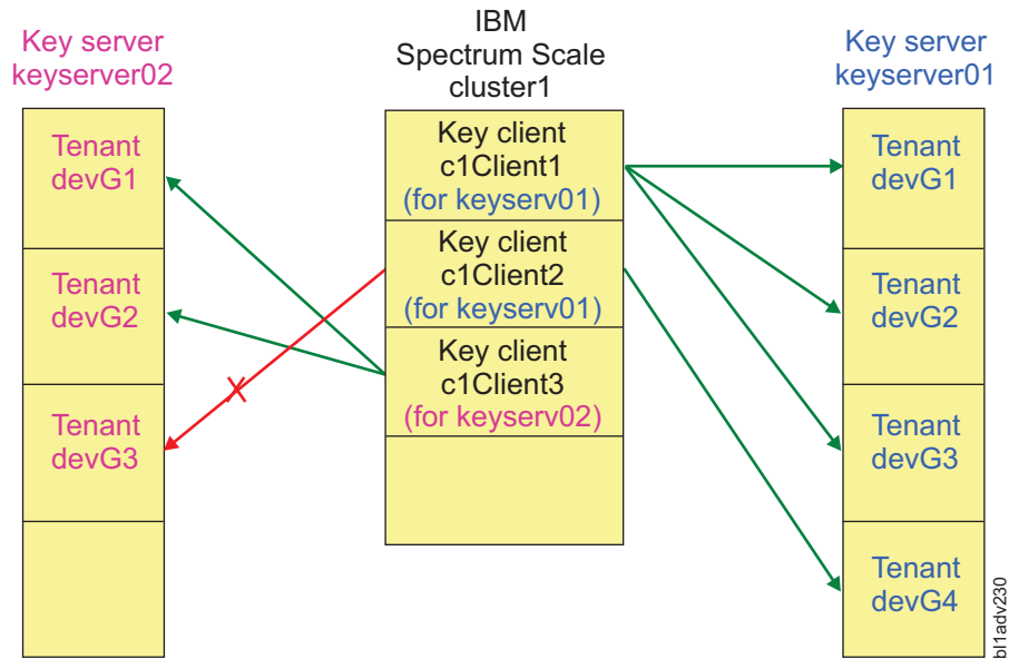
Figure 25. Single cluster, multiple key servers
