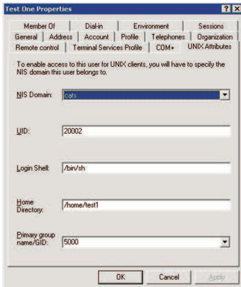
Figure 14. Properties window
