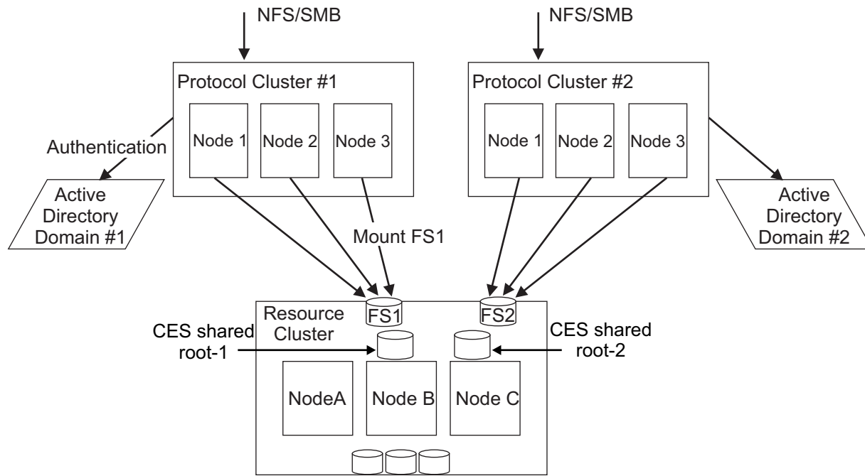
Figure 9. High-level flow of protocols on remotely mounted file systems
