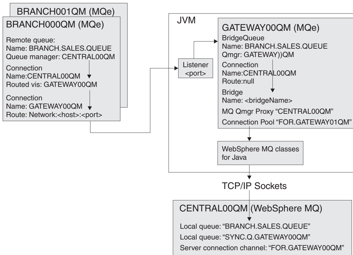
Figure 12. Branch to central routing
