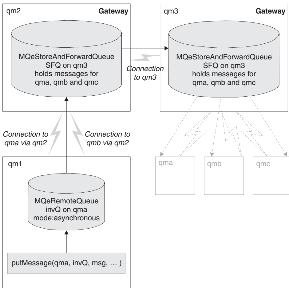
Figure 16. Store-and-forward queue
