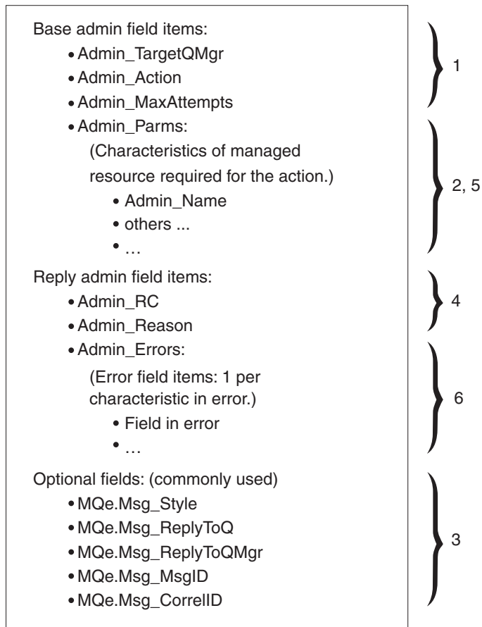
Figure 8. Administration reply message
