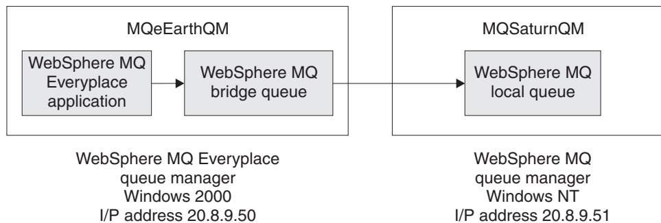
Figure 5. MQ bridge queue
