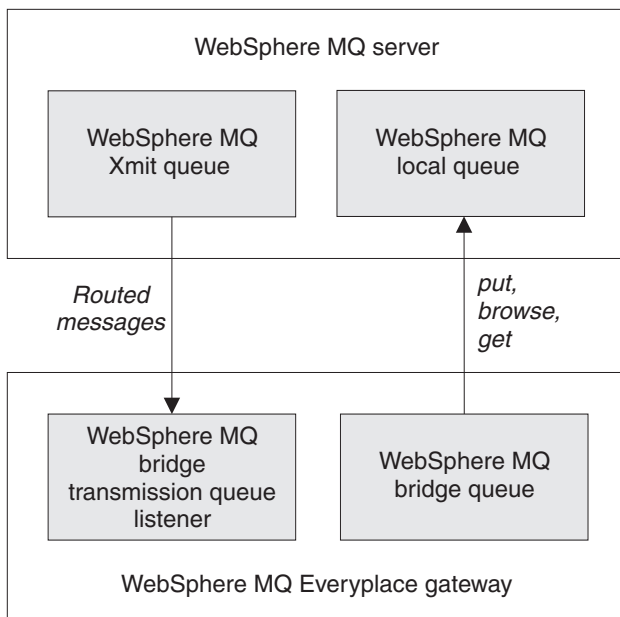
Figure 17. Bridge configuration
