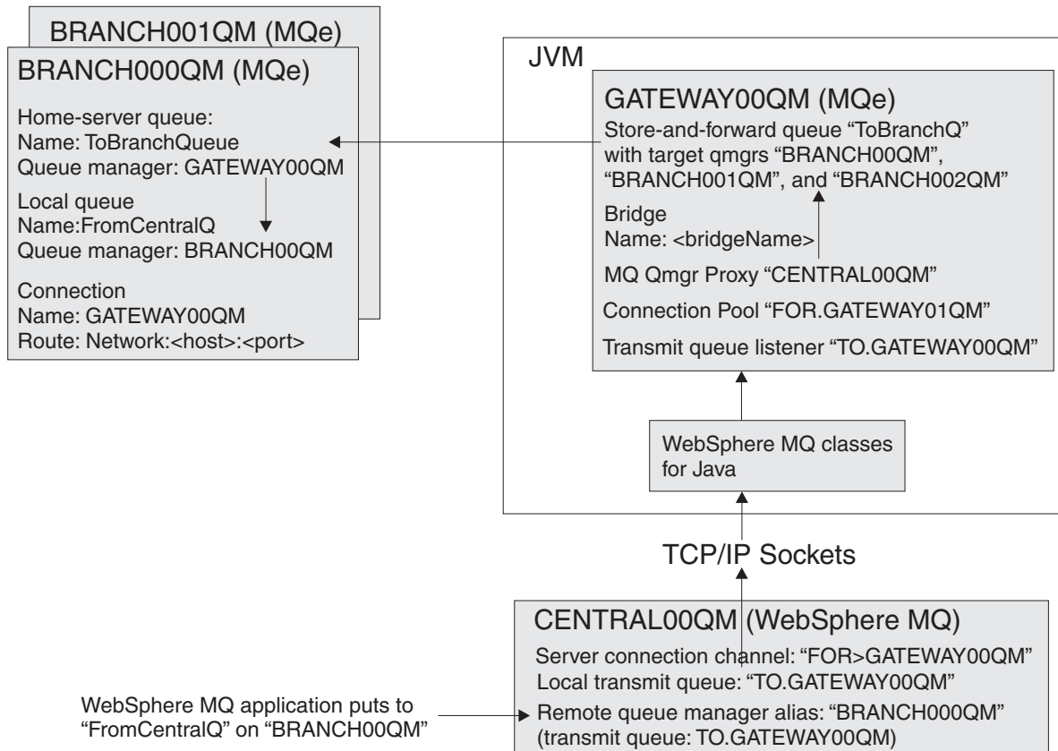
Figure 13. Central to branch routing
