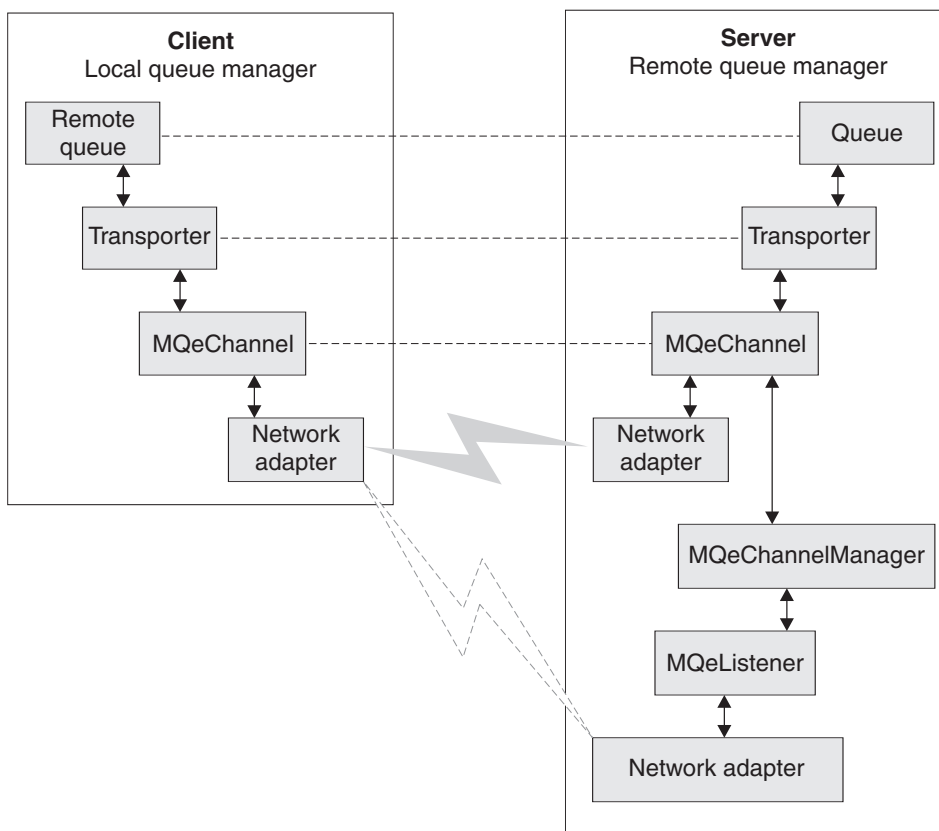
Figure 2. Client to server connections
