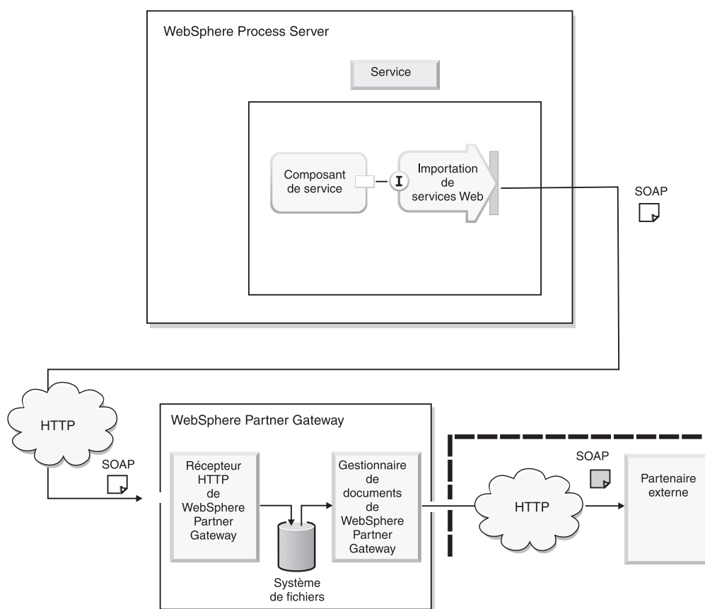
Figure 27. Service de WebSphere Process Server appelant un service Web
