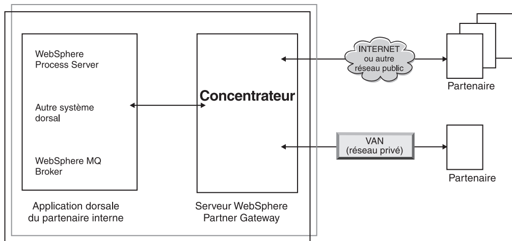
Figure 1. Flux de document complet
