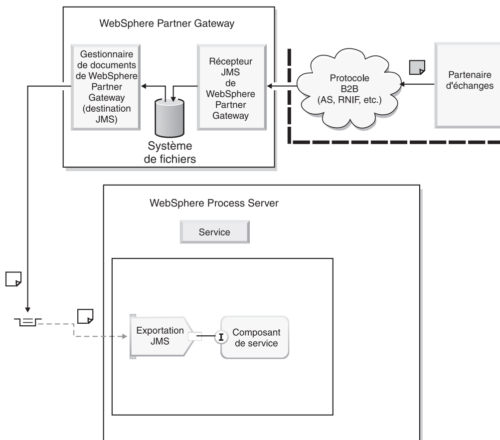
Figure 23. Exportation JMS d'appel des services SCA via JMS
