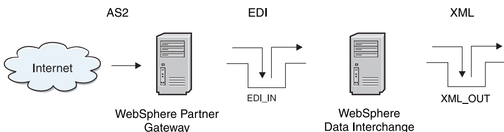
Figure 40. Document EDI provenant de WebSphere Partner Gateway
