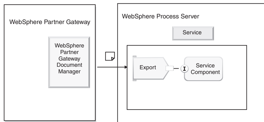
Figure 16. How WebSphere Partner Gateway uses the export binding to send documents to WebSphere Process Server
