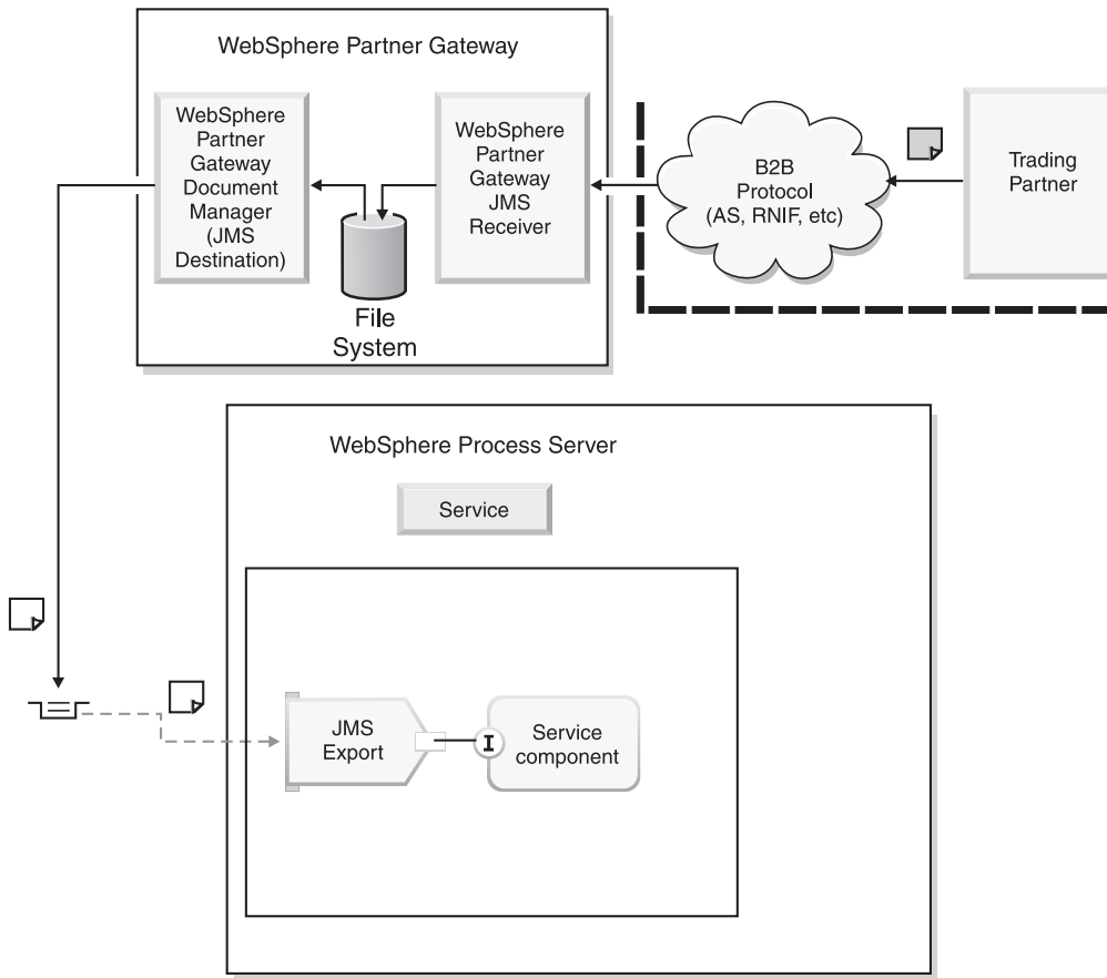
Figure 23. JMS Export to invoke SCA services over JMS
