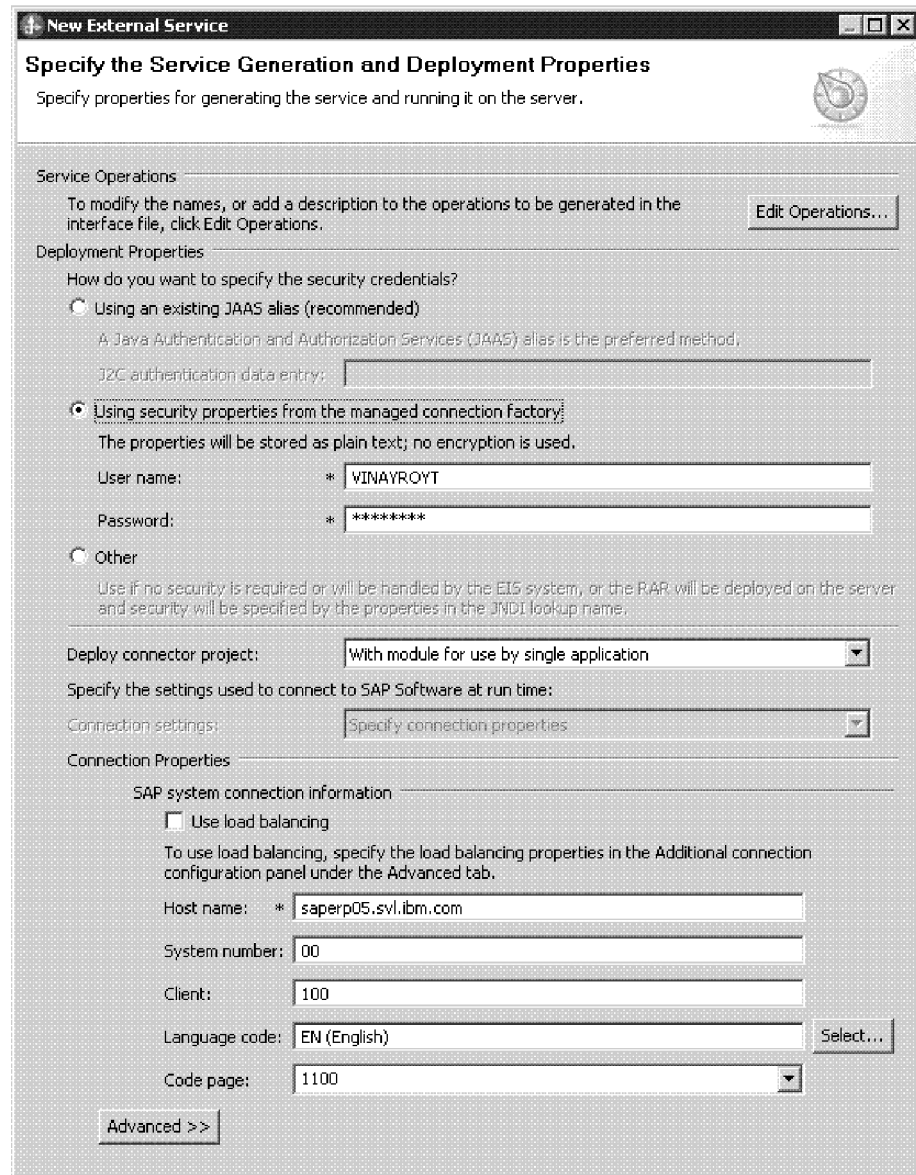
Figure 59. Connection properties
