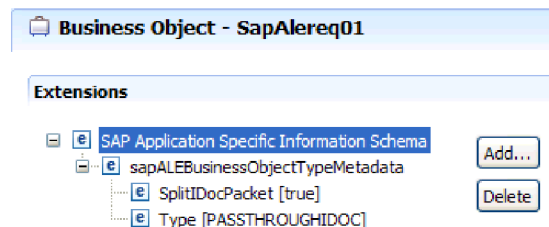
Figure 44. Application-specific information for an ALE pass-through IDoc business object
