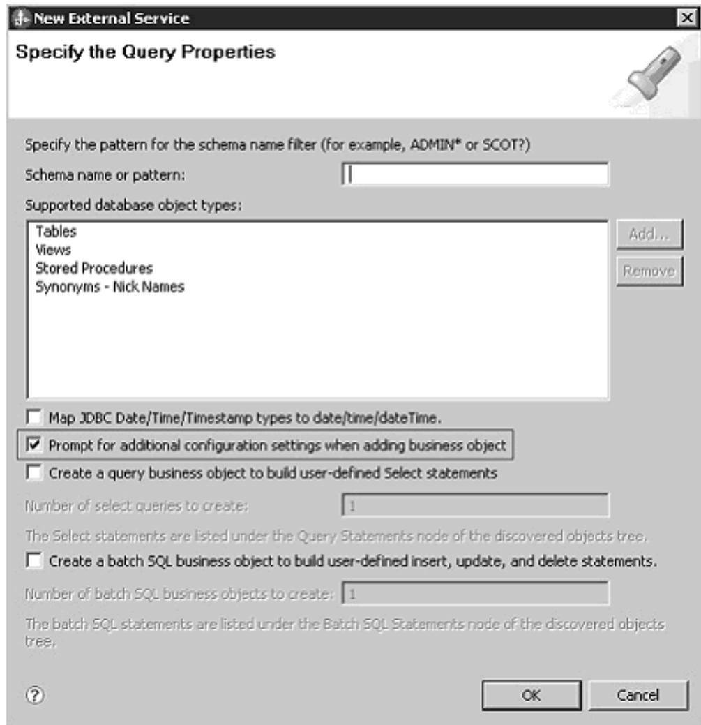
Figure 38. New External Service window
