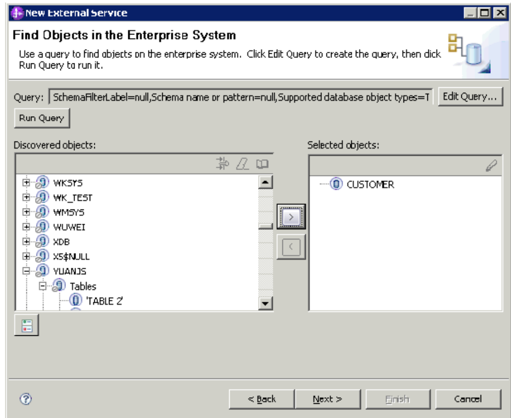
Figure 39. Discovered and Selected objects
