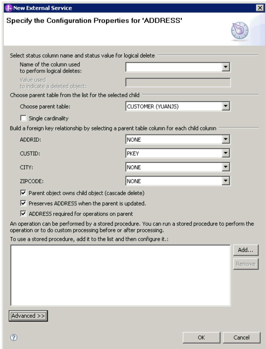
Figure 40. Specifying the Configuration Properties for ADDRESS
