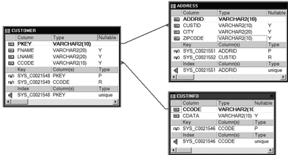
Figure 37. Database Tables
