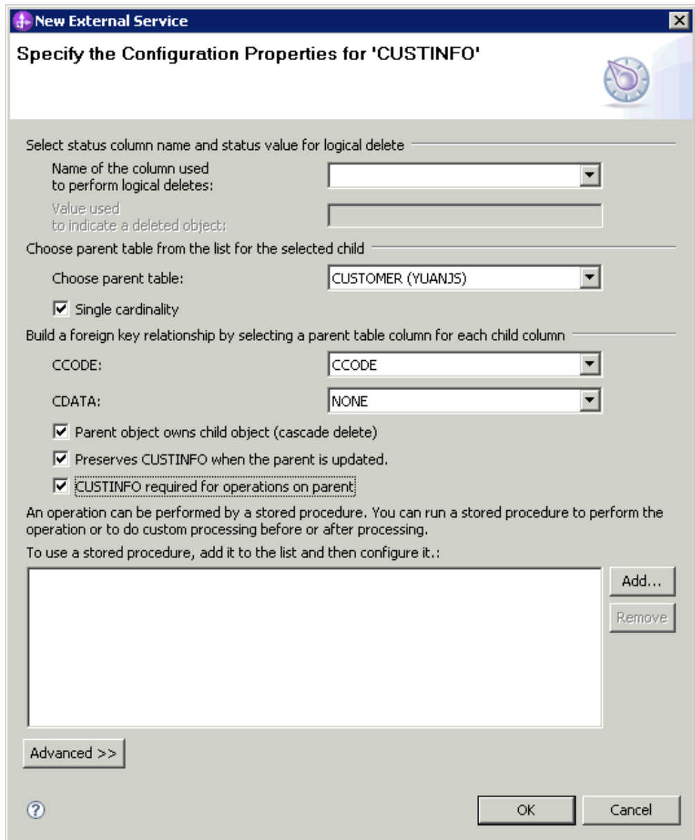
Figure 43. Specifying the Configuration Properties for CUSTINFO
