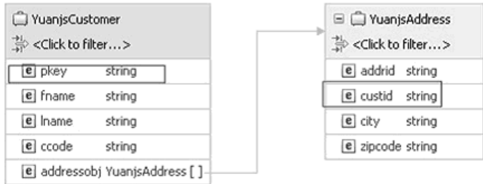
Figure 41. Multiple Cardinality Relationship
