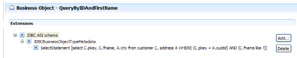
Figure 15. The SELECT statement is saved in the business object application-specific information
