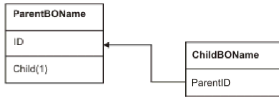
Figure 22. Multiple cardinality relationship with N=1
