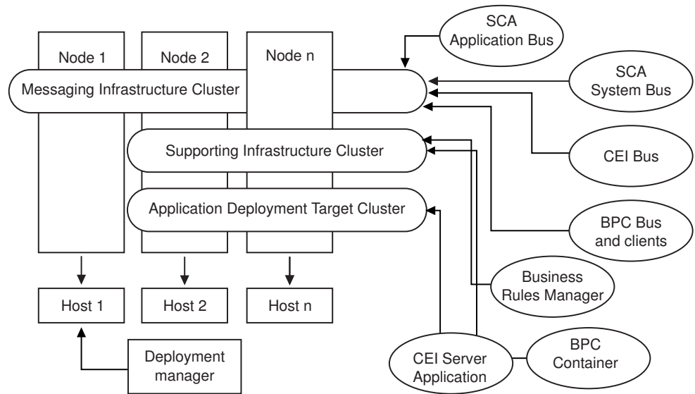
Rysunek 7. Remote messaging and remote support pattern
