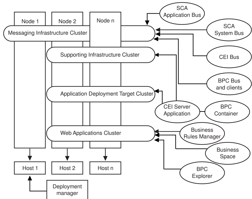
Rysunek 9. Remote messaging, support and web pattern
