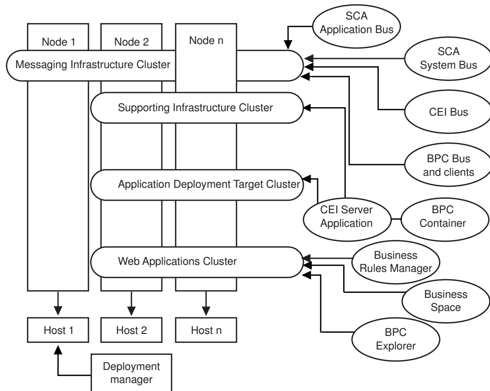
Figure 9. Remote messaging, support and web pattern
