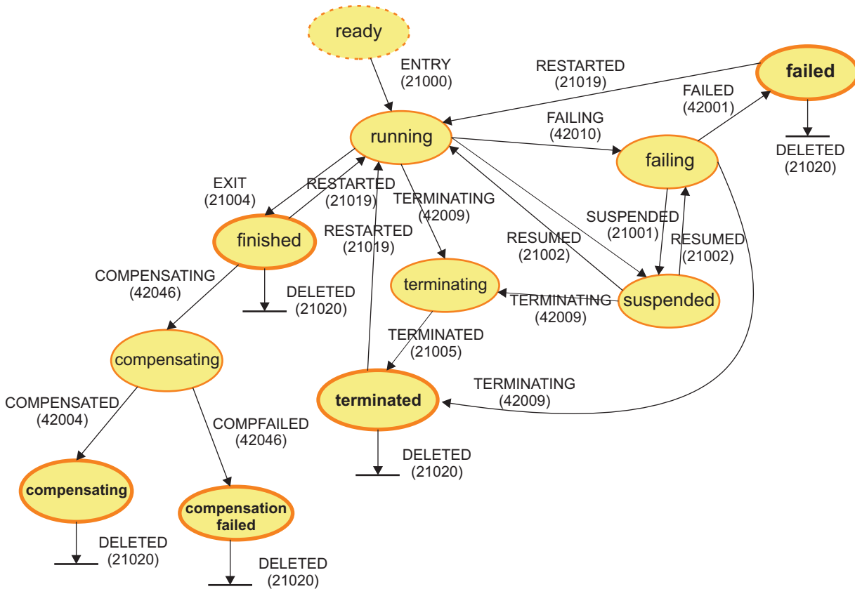
Figure 1. State transitions and process events
