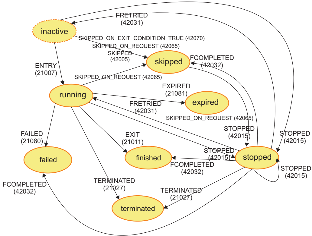
Figure 2. State transitions and events for invoke activities and short-lived activities
