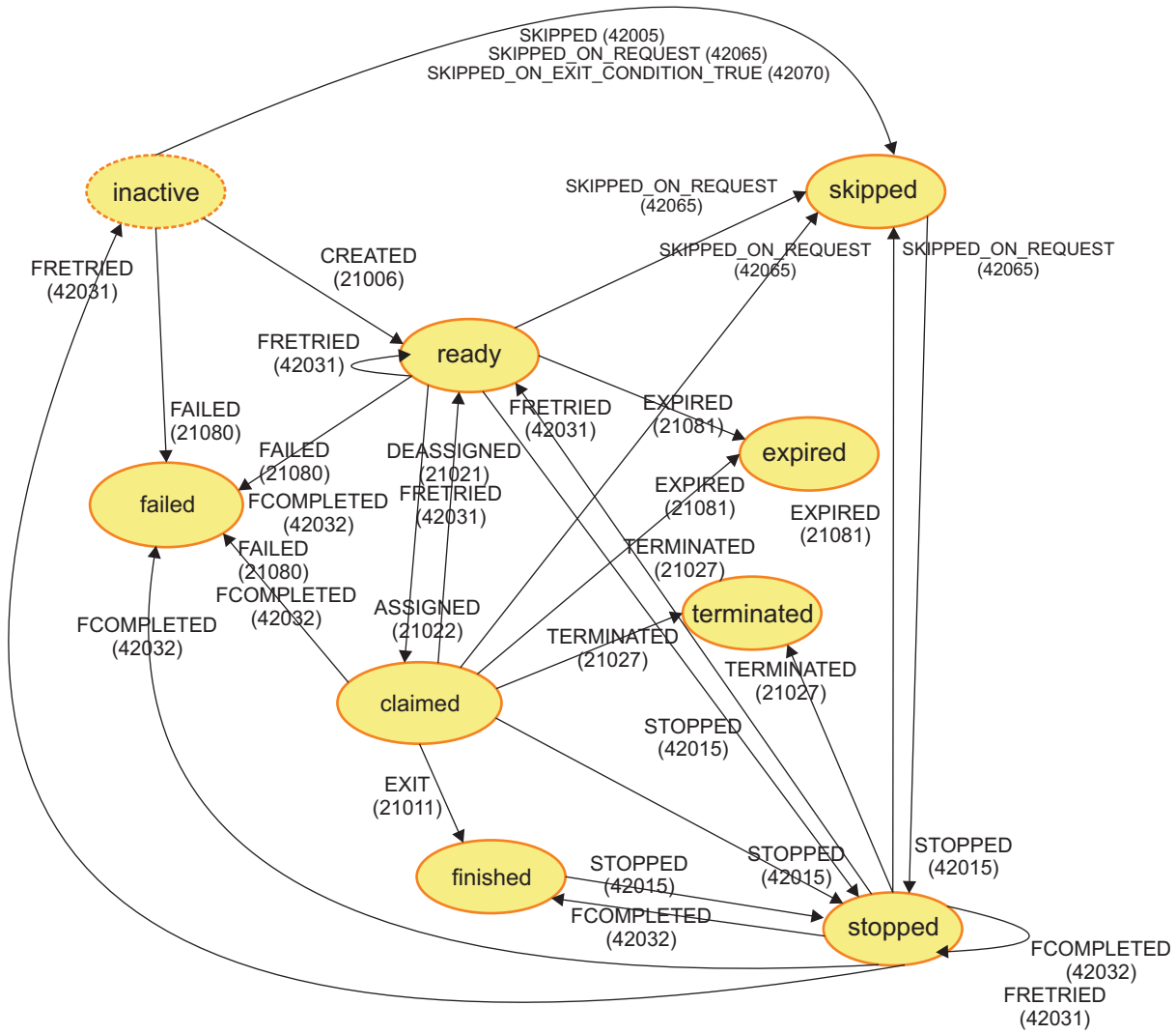
Figure 4. State transitions and events for human task activities
