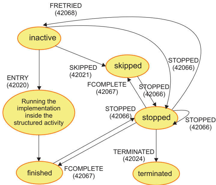
Figure 5. State transitions and events for structured activities
