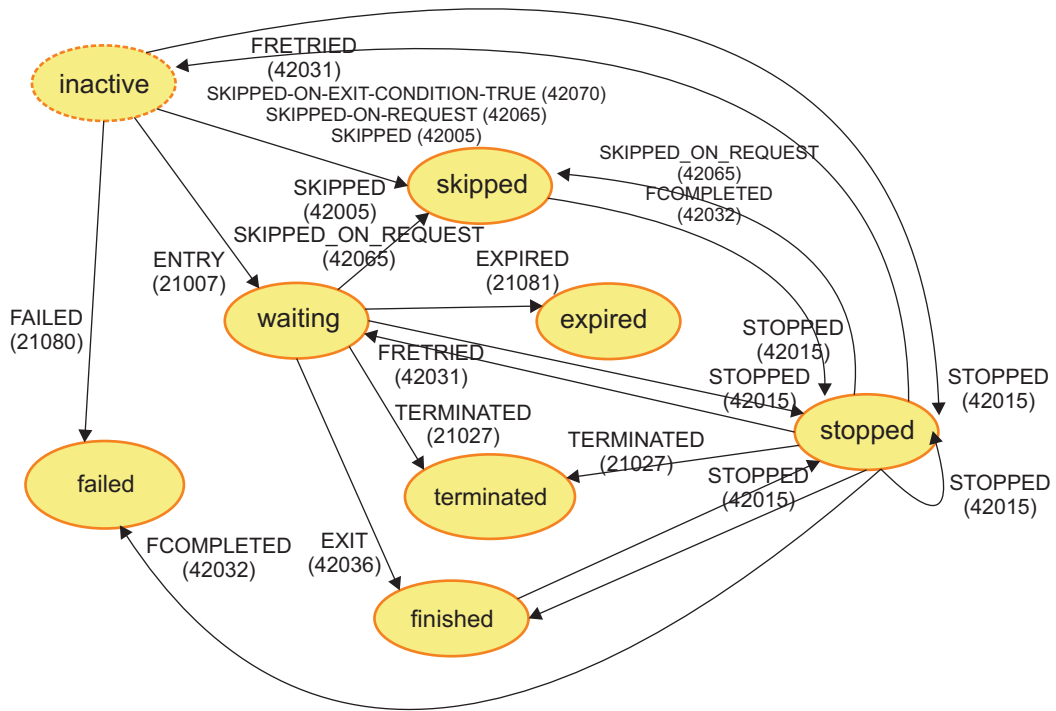
Figure 3. State transitions and events for wait, and receive activities
