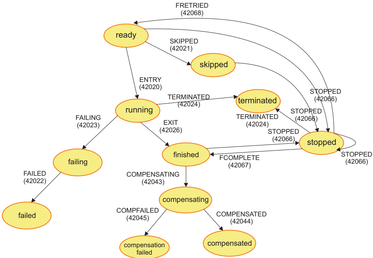
Figure 6. State transitions and events for scope activities
