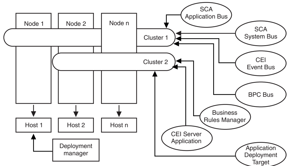
Figure 2. Remote messaging pattern
