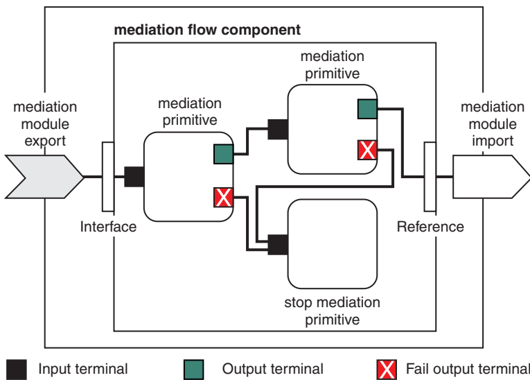
Figure 10. Simplified example of a mediation module. The mediation module contains one mediation flow component, which contains mediation primitives.
