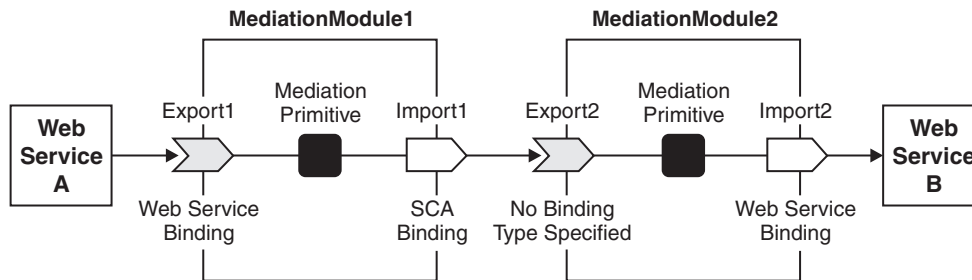
Figure 12. Example showing one mediation module interacting with another mediation module. Mediation Module1 connects to Mediation Module2
