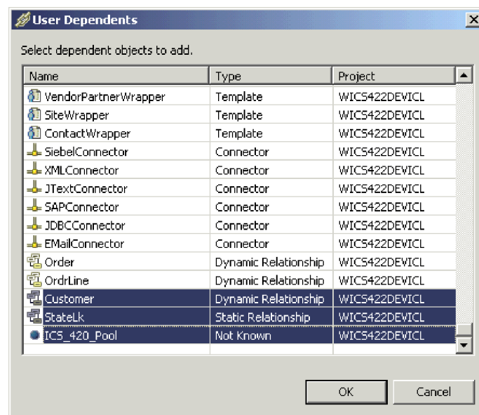
Figure 78. Adding user dependents
