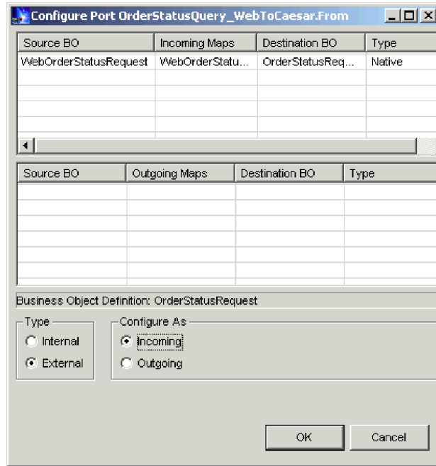
Figure 60. Configuring external collaboration object ports
