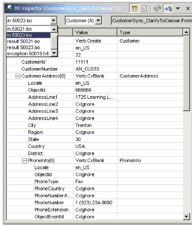
Figure 89. Business object inspector view
