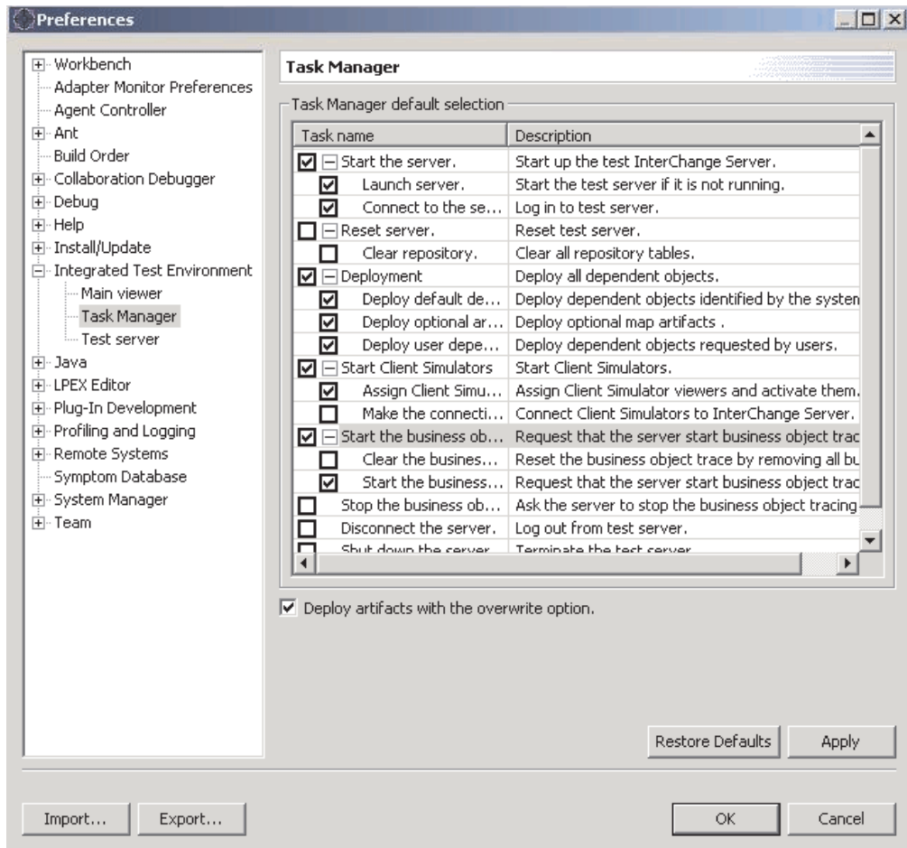
Figure 79. Task Manager view
