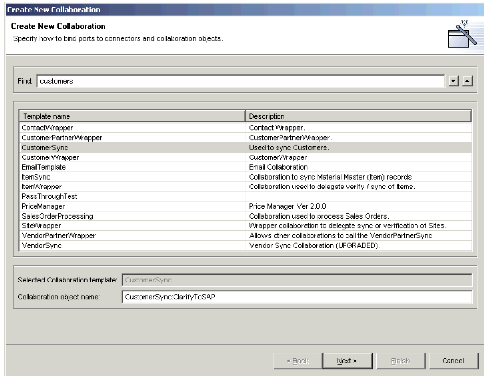
Figure 53. Using the Find field
