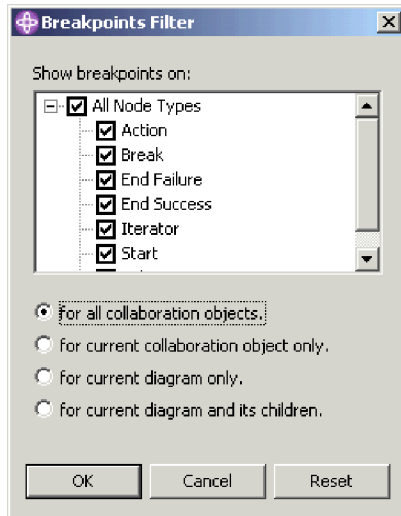
Figure 103. Breakpoints filter
