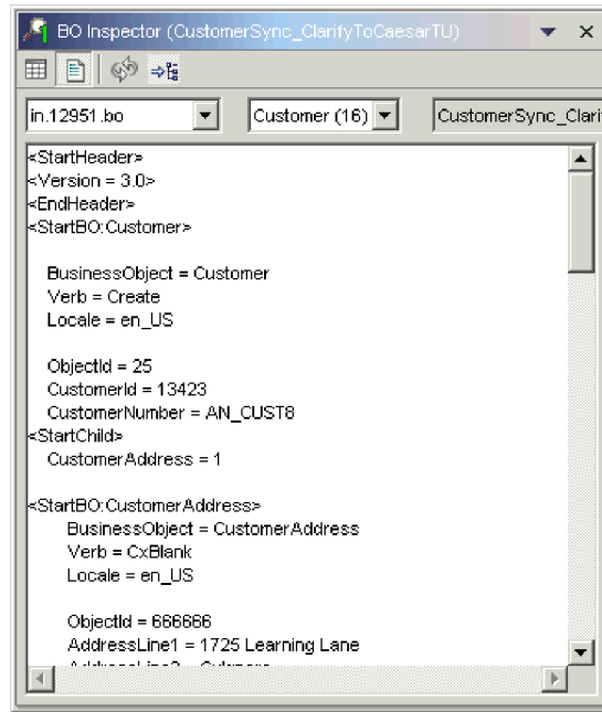
Figure 90. BO Inspector view with business object data in text view style
