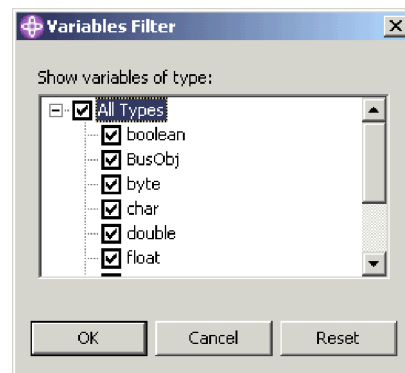
Figure 104. Variables filter
