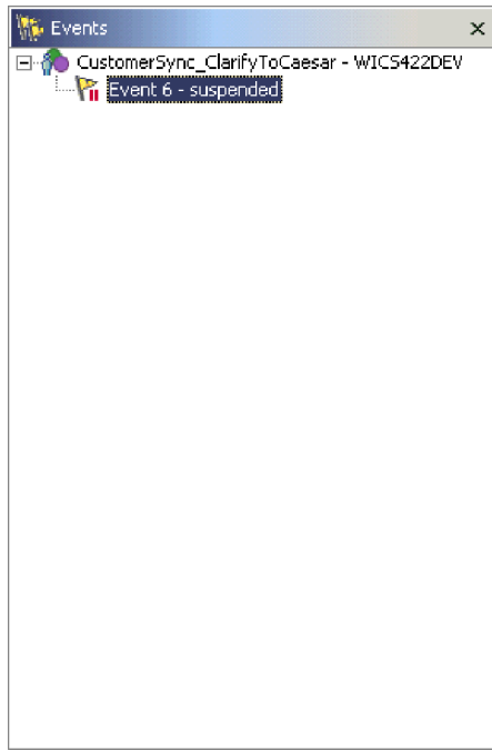
Figure 96. Events view
