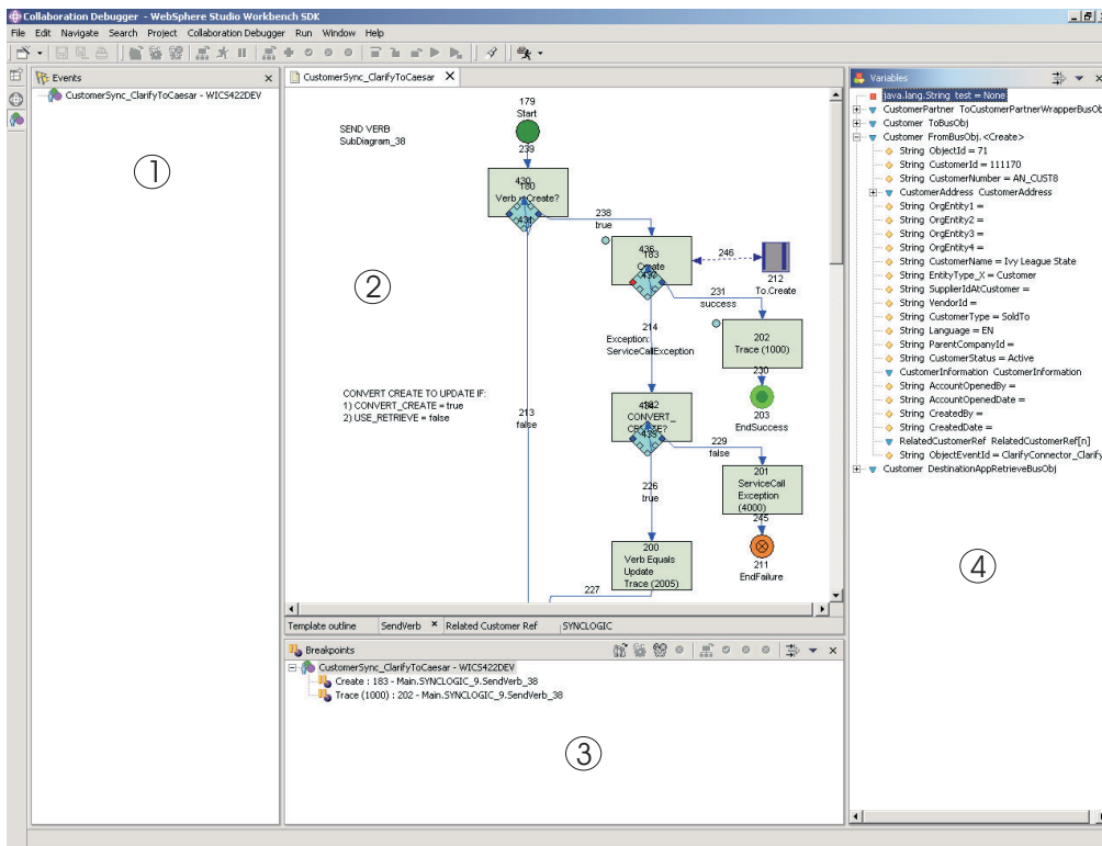
Figure 95. Collaboration Debugger perspective
