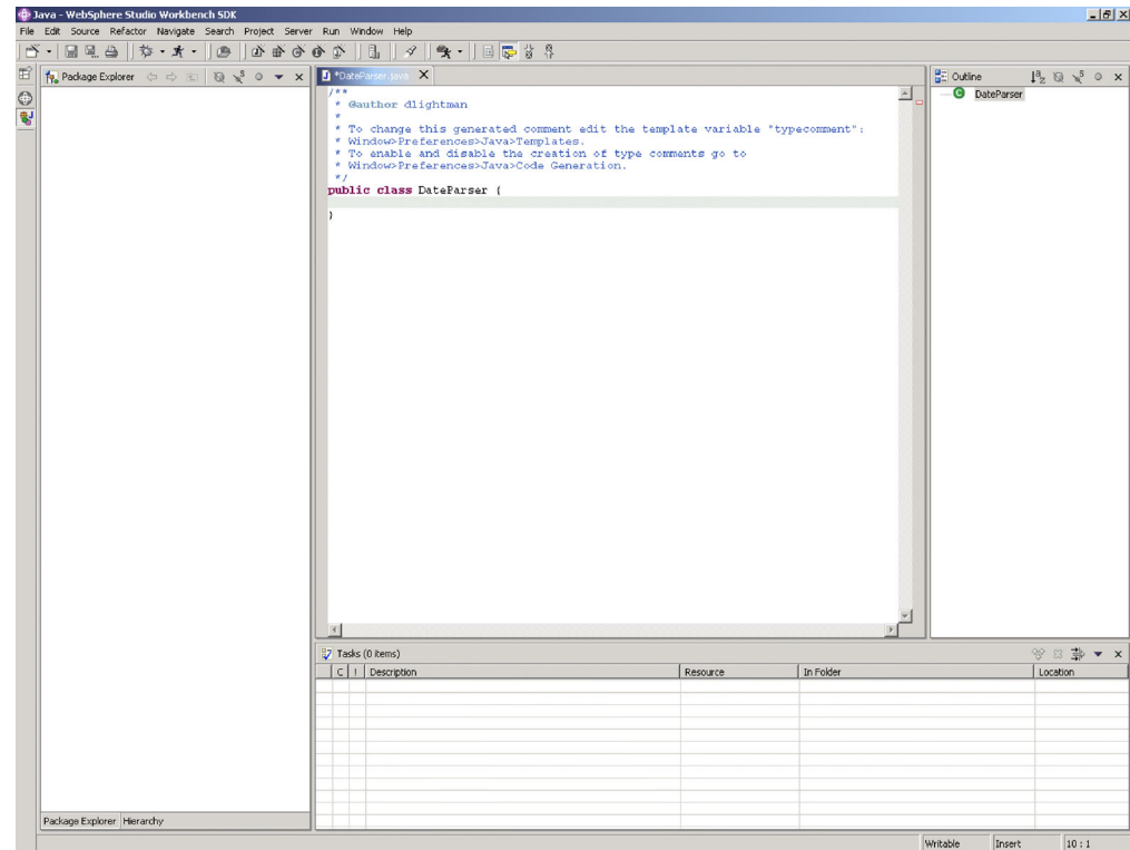
Figure 30. Java perspective
