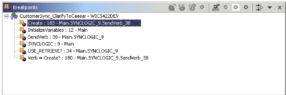
Figure 98. Breakpoints view
