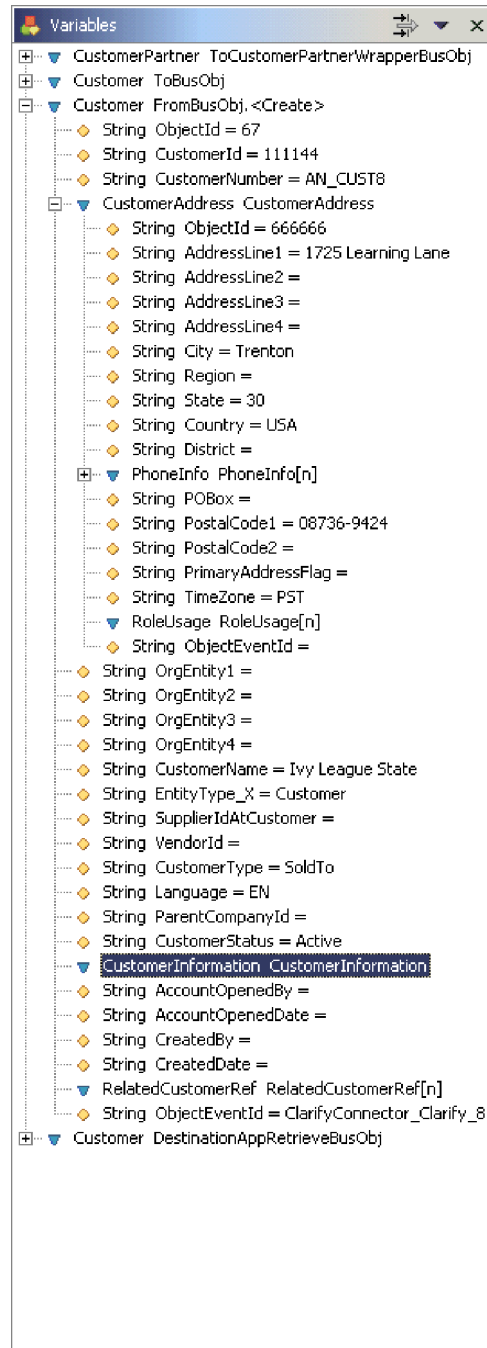
Figure 99. Variables view
