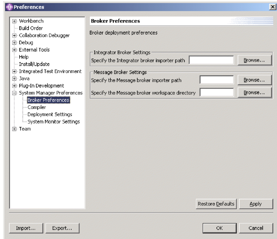
Figure 32. Broker preferences
