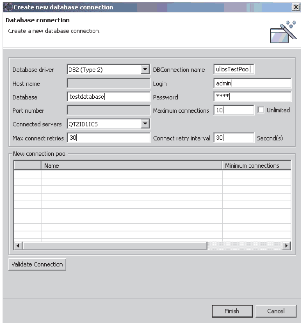
Figure 50. Create New Database Connection wizard
