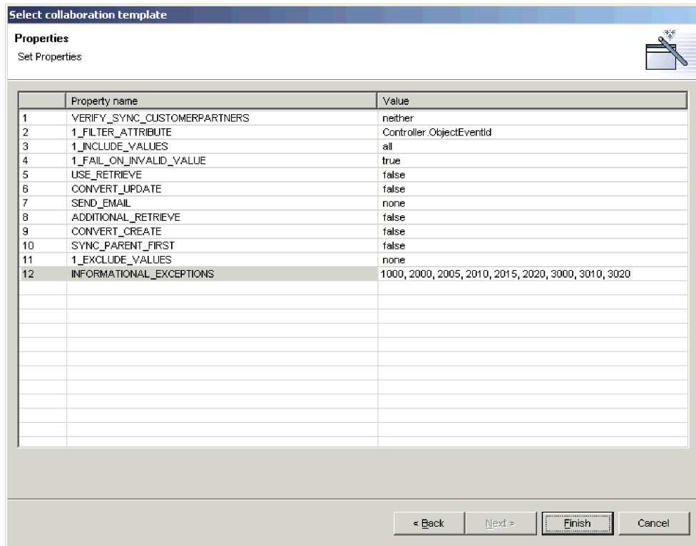
Figure 56. Configuring collaboration template-specific properties
