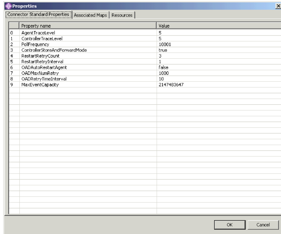
Figure 26. Modifying connector properties
