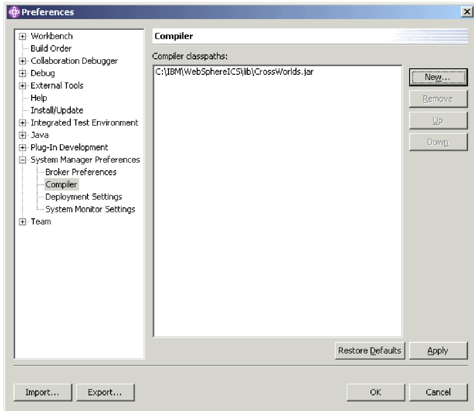
Figure 33. Compiler preferences
