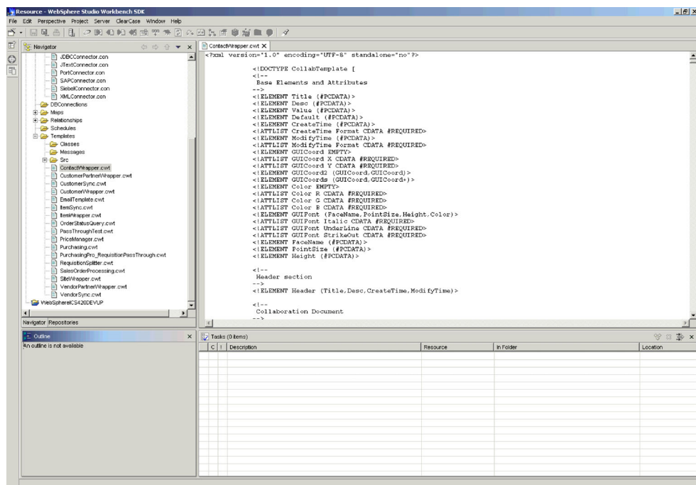
Figure 29. Resource perspective
