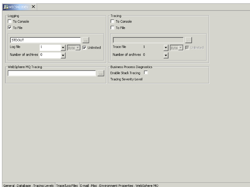
Figure 43. Configuring InterChange Server logging and tracing properties
