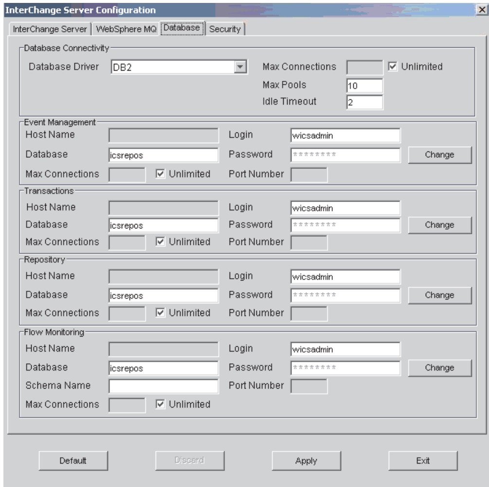
Figure 38. Database connectivity configuration tab
