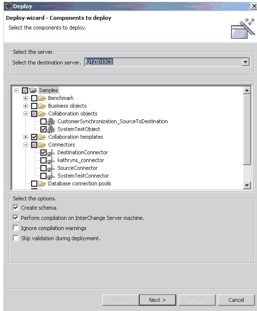
Figure 20. Selecting deployable components and deployment options
