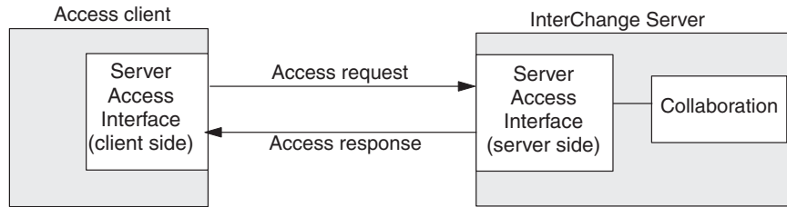
Figure 1. Call-triggered flow
