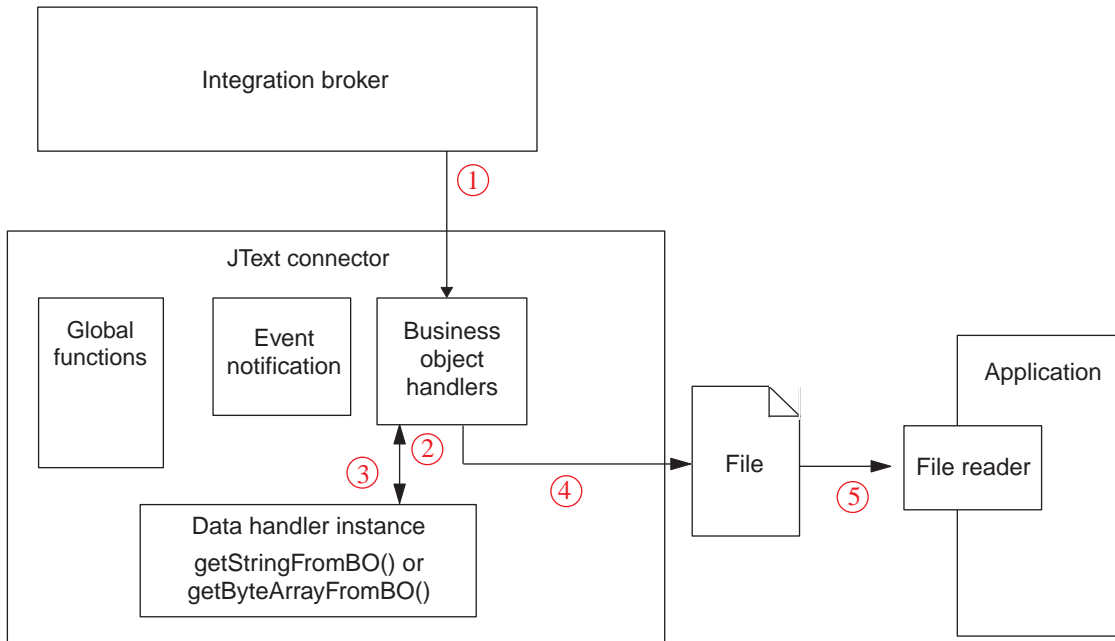
Figure 4. Business object request operation
