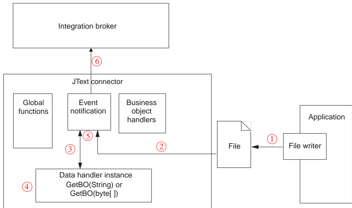
Figure 3. Event notification operation
