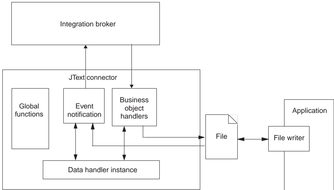
Figure 1. JText connector architecture
