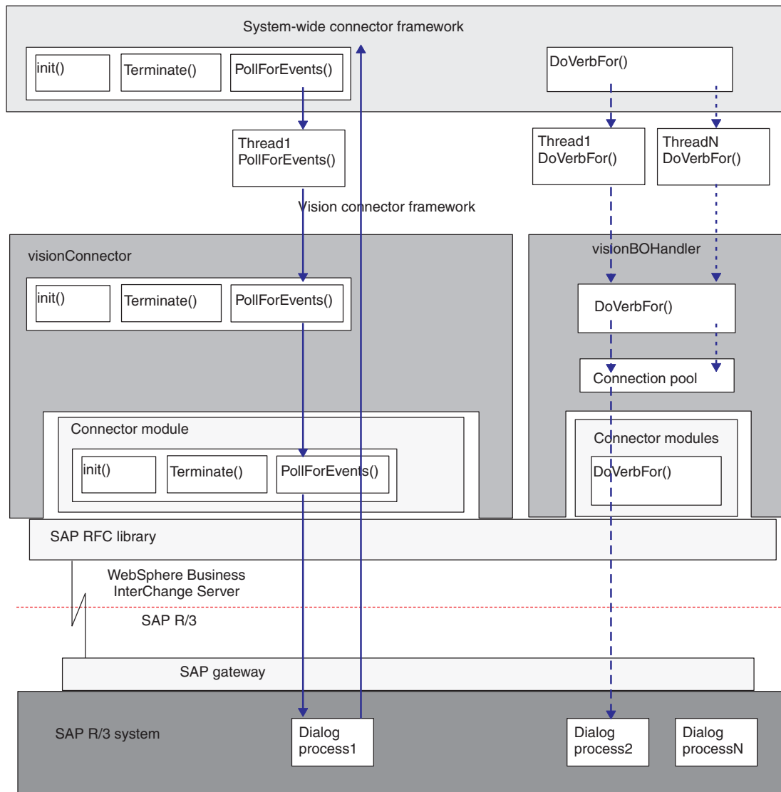
Figure 4. Multi-Threading architecture of the connector for SAP
