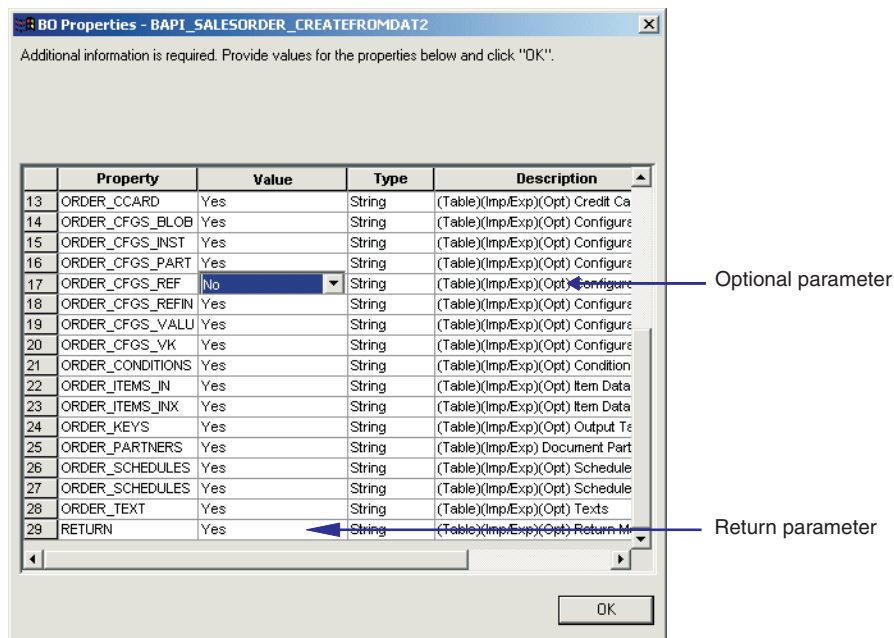
Figure 16. Specifying attributes for removal from the definition
