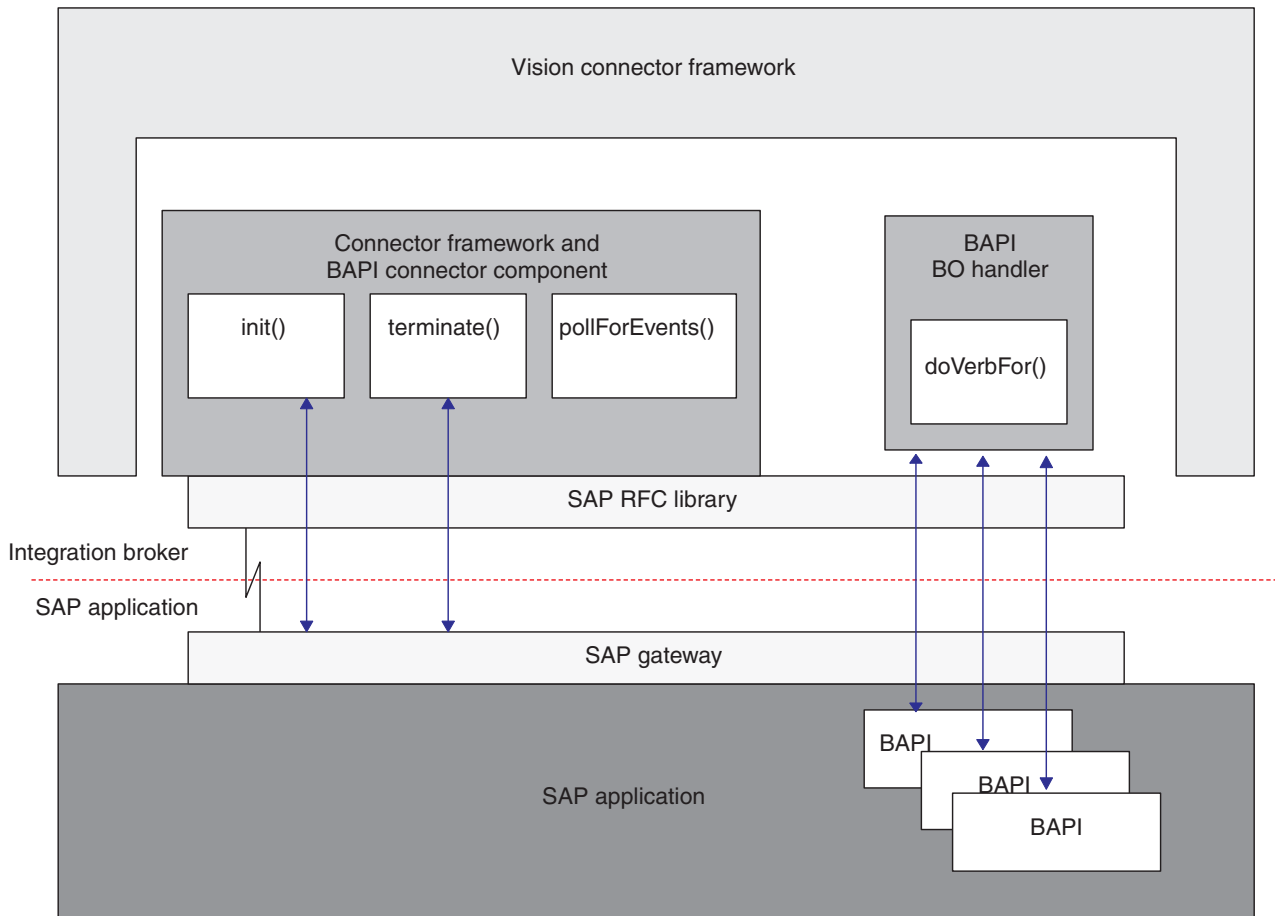
Figure 46. BAPI Module architecture
