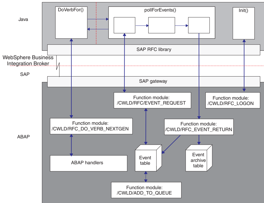
Figure 64. ABAP Extension Module architecture
