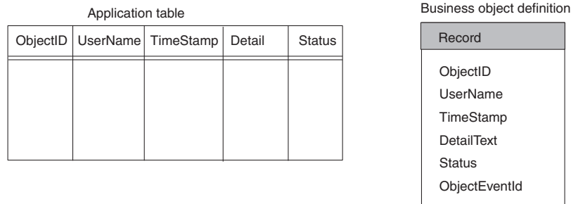
Figure 8. Flat business object representing one entity
