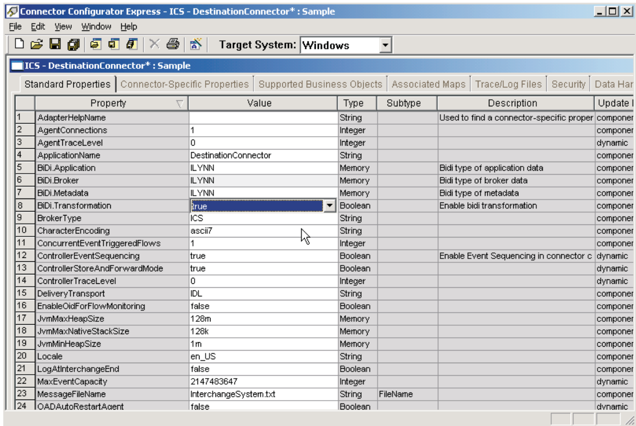
Figure 18. The BiDiTransformation property in the Connector Configurator Express
