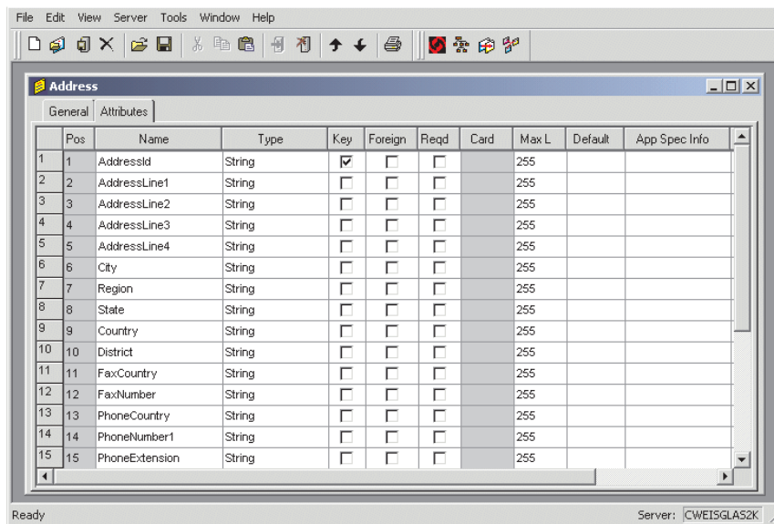
Figure 28. Defining and editing attributes
