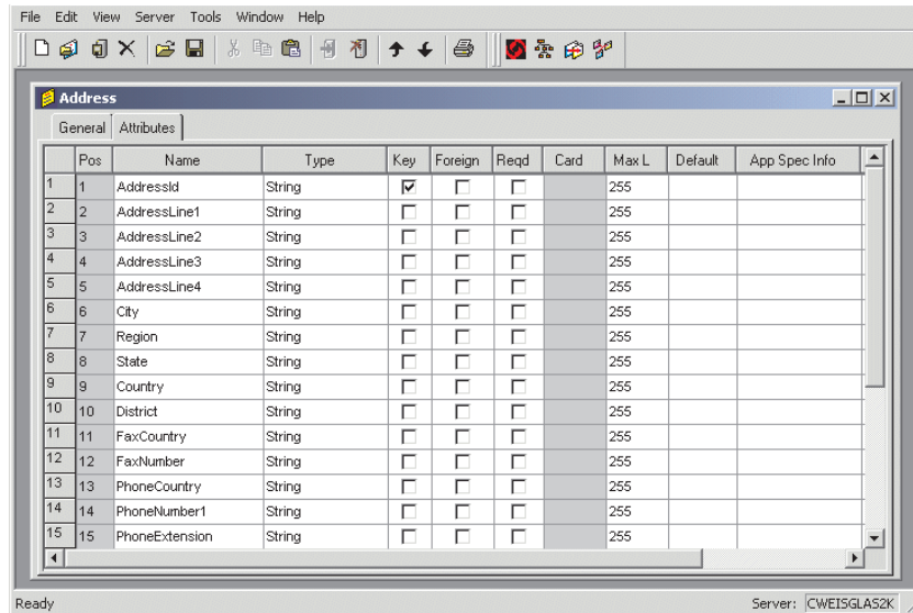
Figure 33. Initial display of a new business object definition
